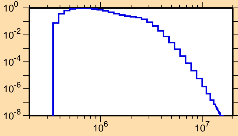
\sigma vs. E for ^{95}\text{Sr}(n,n_1)
