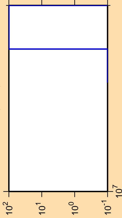
\Delta\sigma/\sigma vs. E for ^{95}\text{Sr}(n,\text{nd})
