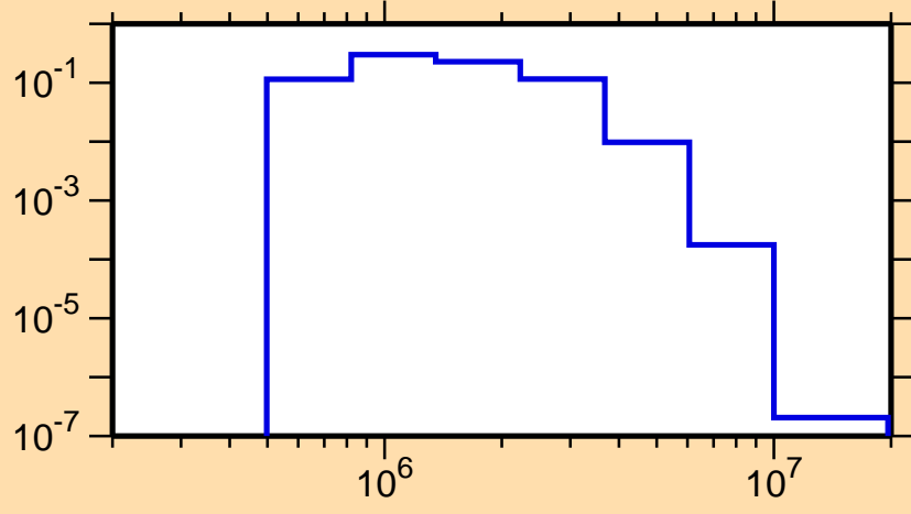
\sigma vs. E for ^{95}\text{Sr}(n,n_2)
