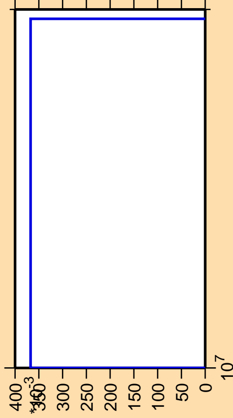
\Delta\sigma/\sigma vs. E for ^{95}\text{Sr}(n,2np)
