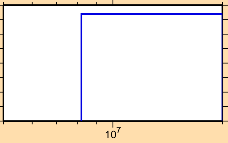
\sigma vs. E for ^{95}\text{Sr}(n,\alpha)
