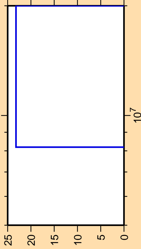
\Delta\sigma/\sigma vs. E for ^{95}\text{Sr}(n,3n)
