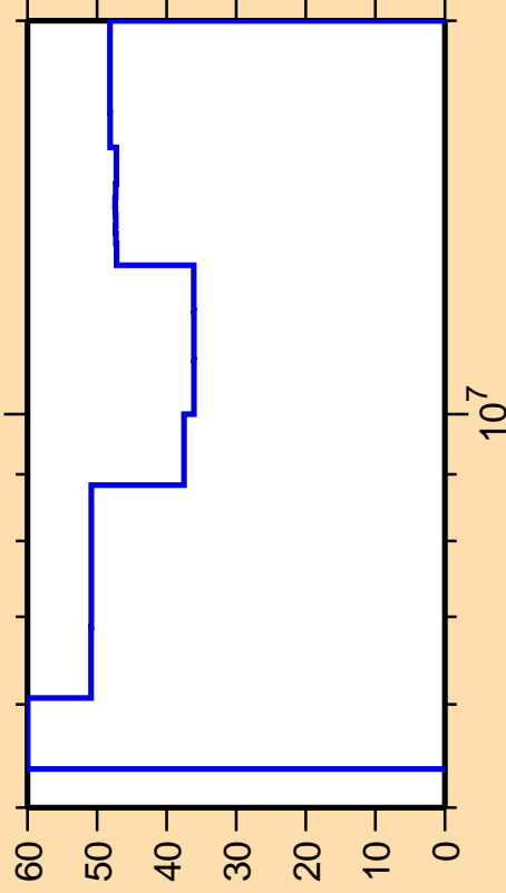
\Delta\sigma/\sigma vs. E for ^{96}\text{Sr}(n,2n)
