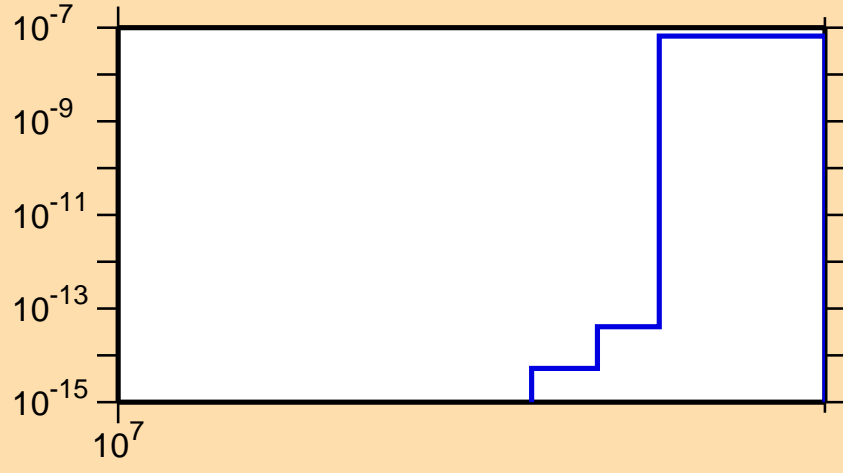
\sigma vs. E for ^{96}\text{Sr}(n,nt)
