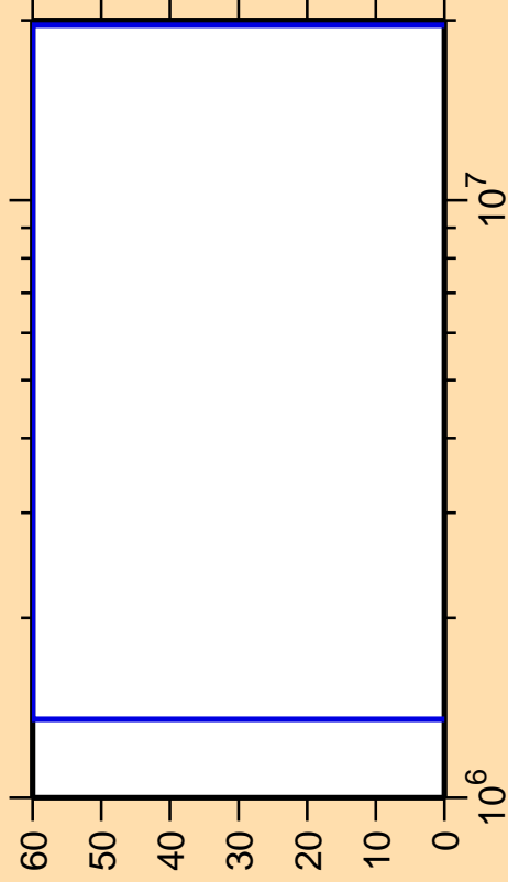
\Delta\sigma/\sigma vs. E for ^{96}\text{Sr}(n,n_3)
