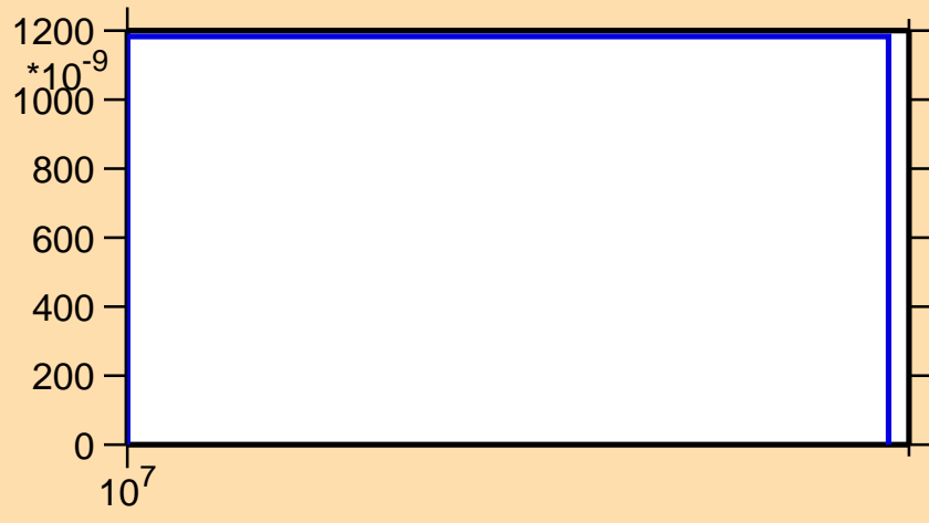
\sigma vs. E for ^{96}\text{Sr}(n,t)
