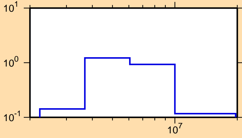
\sigma vs. E for ^{96}\text{Sr}(n,n\text{cont.})
