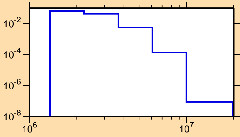
\sigma vs. E for ^{96}\text{Sr}(n,n_3)
