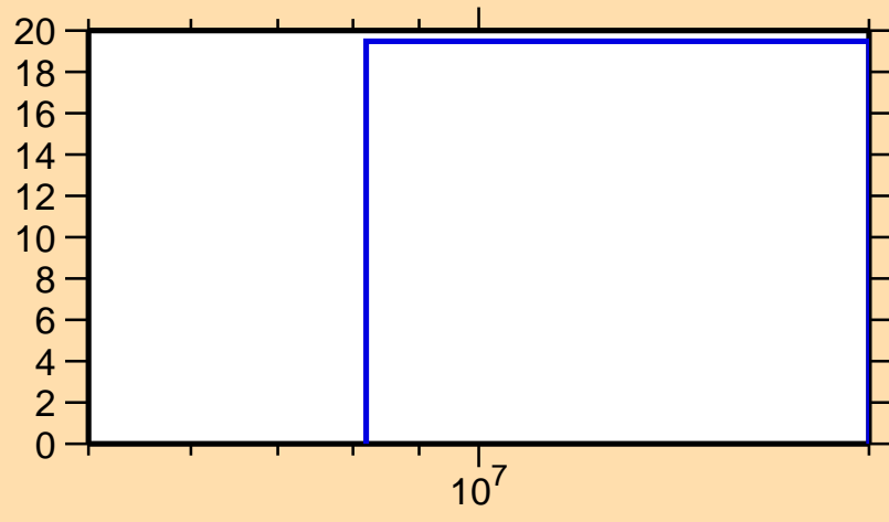
\Delta\sigma/\sigma vs. E for ^{96}\text{Sr}(n,el.)
