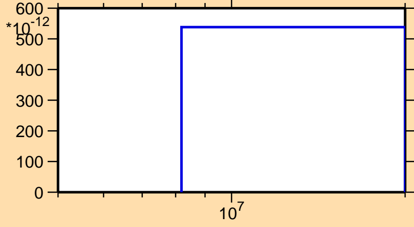
\sigma vs. E for ^{96}\text{Sr}(n,nt)
