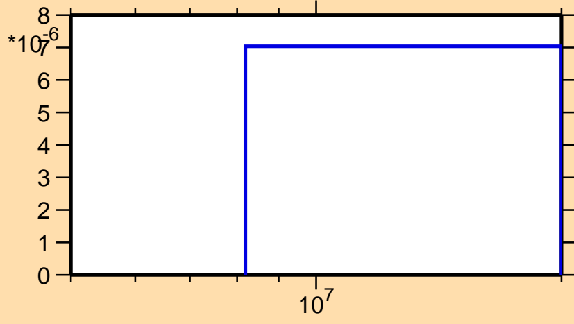
\sigma vs. E for ^{96}\text{Sr}(n,p)
