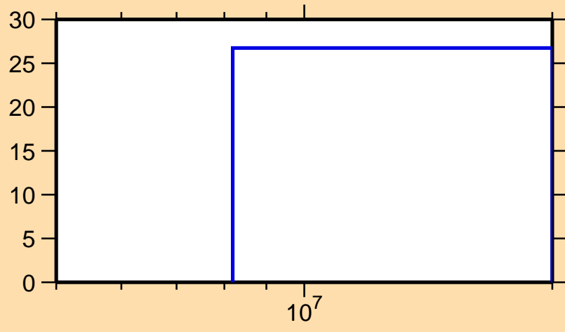
\Delta\sigma/\sigma vs. E for ^{96}\text{Sr}(n,\text{nonel.})
