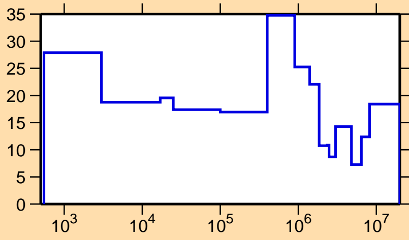
\Delta\sigma/\sigma vs. E for ^{96}\text{Sr}(n,\text{tot.})
