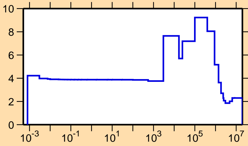
\sigma vs. E for ^{96}\text{Sr}(n,\text{el.})
