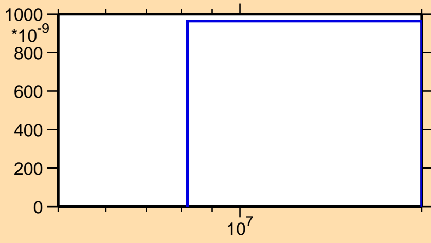
\sigma vs. E for ^{96}\text{Sr}(n,\alpha)
