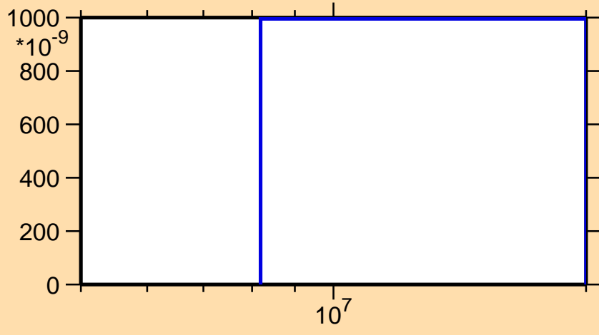
\sigma vs. E for ^{96}\text{Sr}(n,d)
