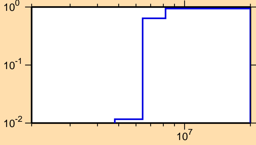
\sigma vs. E for ^{96}\text{Sr}(n,2n)
