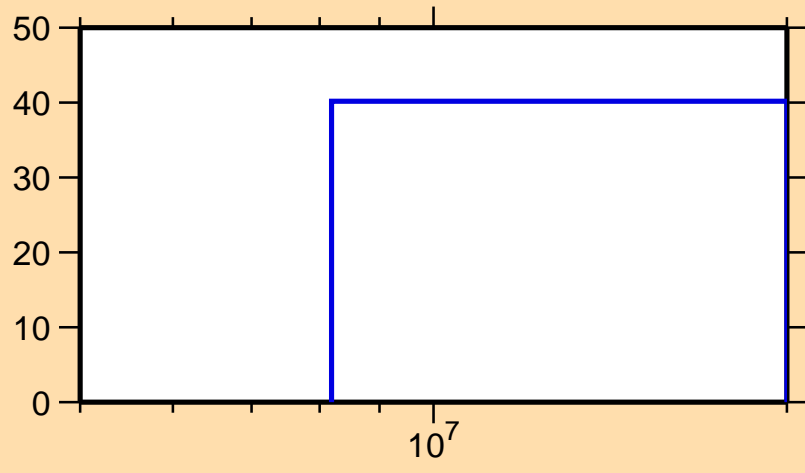
\Delta\sigma/\sigma vs. E for ^{96}\text{Sr}(n,2n)
