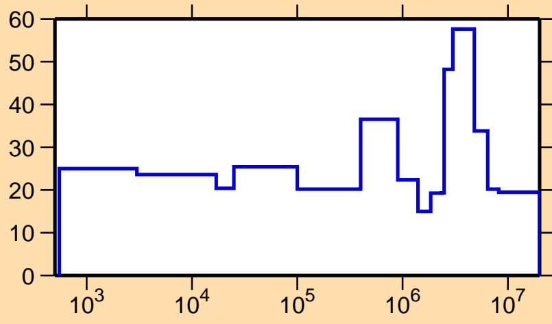
\Delta\sigma/\sigma vs. E for ^{96}\text{Sr}(n,\text{el.})
