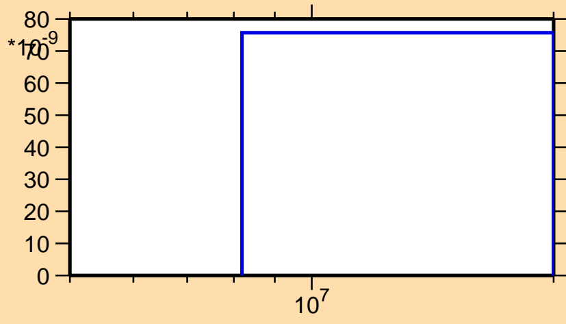
\sigma vs. E for ^{96}\text{Sr}(n,np)
