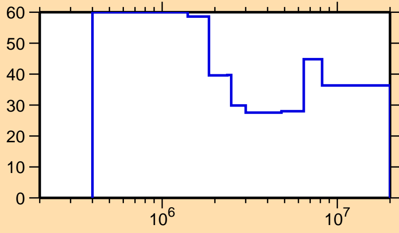
\Delta\sigma/\sigma vs. E for ^{96}\text{Sr}(n,\text{inel.})
