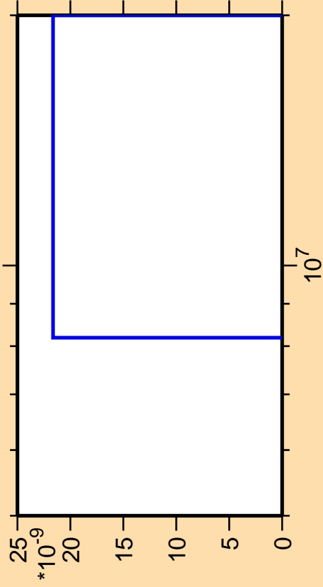
\Delta\sigma/\sigma vs. E for ^{96}\text{Sr}(n,2np)
