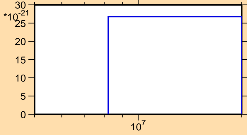
\sigma vs. E for ^{96}\text{Sr}(n,2np)
