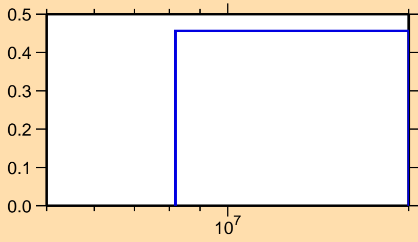
\sigma vs. E for ^{96}\text{Sr}(n,3n)
