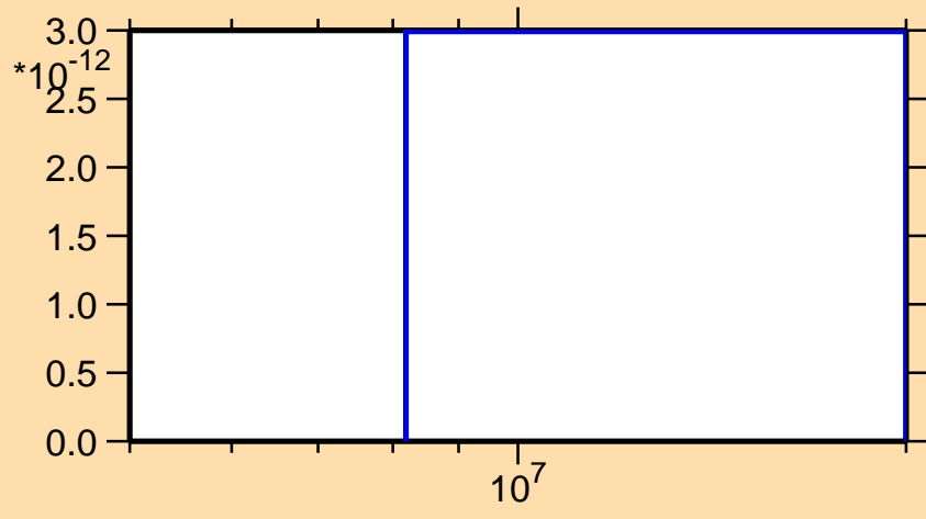
\sigma vs. E for ^{96}\text{Sr}(n,2n\alpha)
