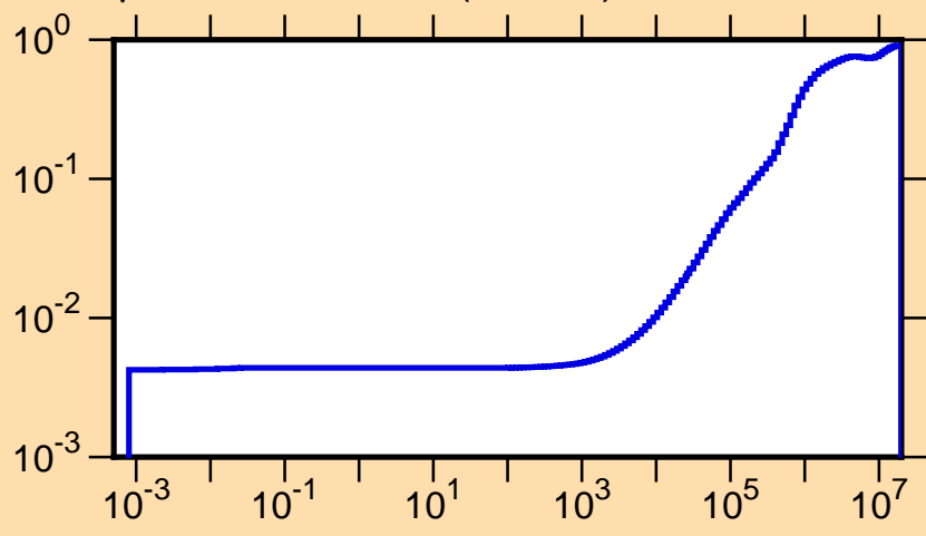
\mu vs. E for ^{159}\text{Ta}(\text{mt251})
