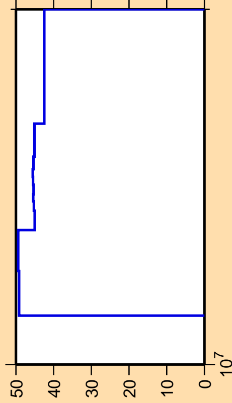
\Delta\sigma/\sigma vs. E for ^{159}\text{Ta}(n,p)
