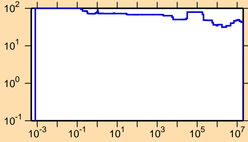
\Delta\sigma/\sigma vs. E for ^{159}\text{Ta}(n,p)
