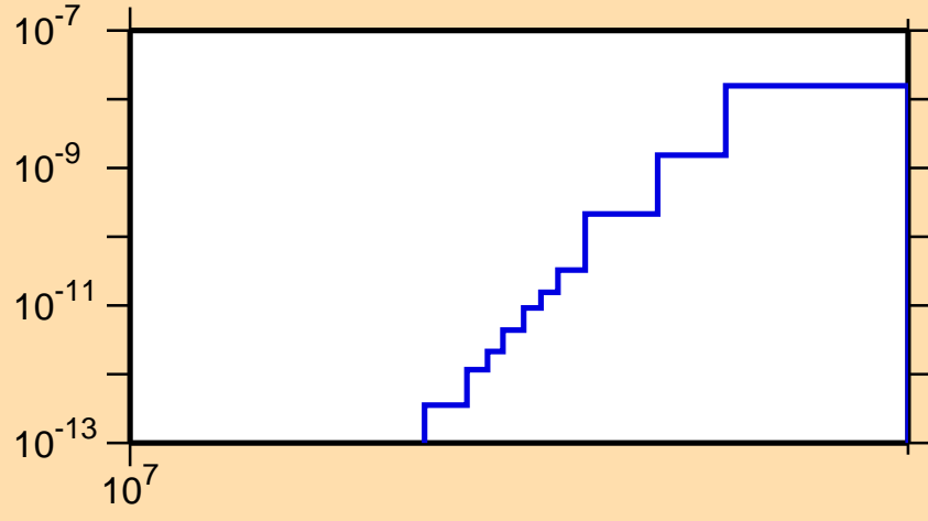
\sigma vs. E for ^{159}\text{Ta} (mt 34)
