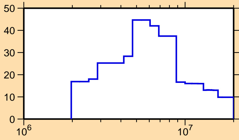
\Delta\sigma/\sigma vs. E for ^{159}\text{Ta}(n,\text{el.})
