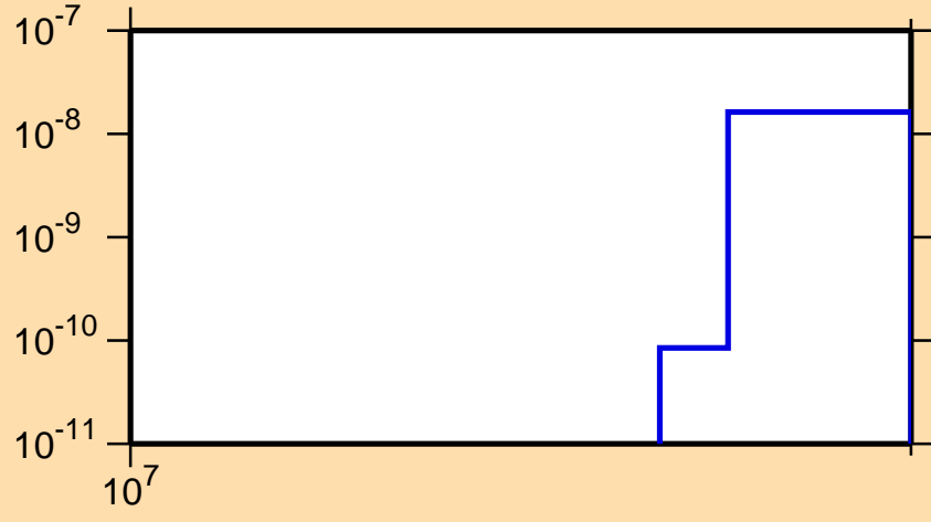
\sigma vs. E for ^{159}\text{Ta}(n,nt)
