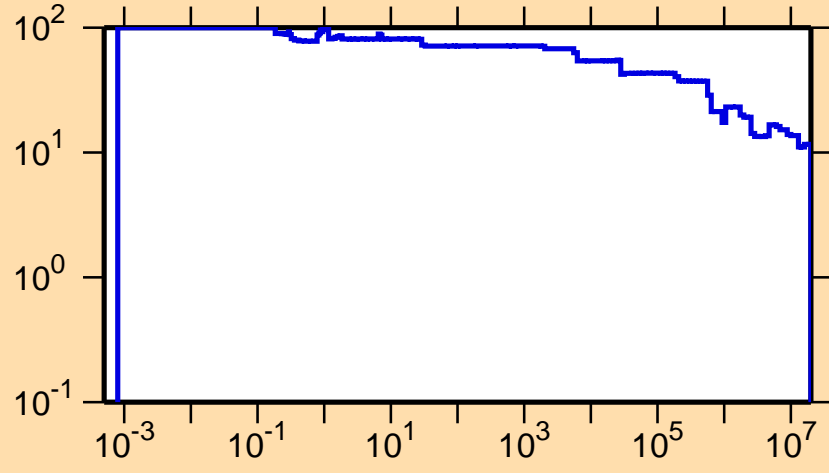
\Delta\sigma/\sigma vs. E for ^{159}\text{Ta}(n,\text{nonel.})
