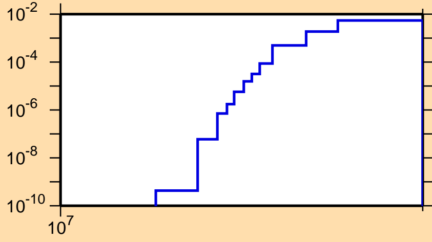
\sigma vs. E for ^{159}\text{Ta}(n,2np)
