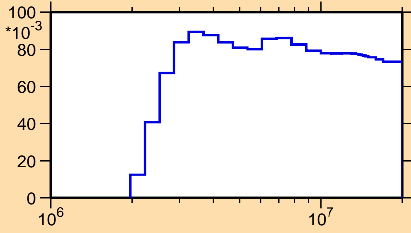
\sigma vs. E for ^{159}\text{Ta}(n,n\text{cont.})
