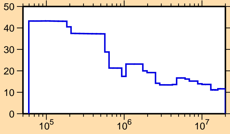
\Delta\sigma/\sigma vs. E for ^{159}\text{Ta}(n,\text{nonel.})
