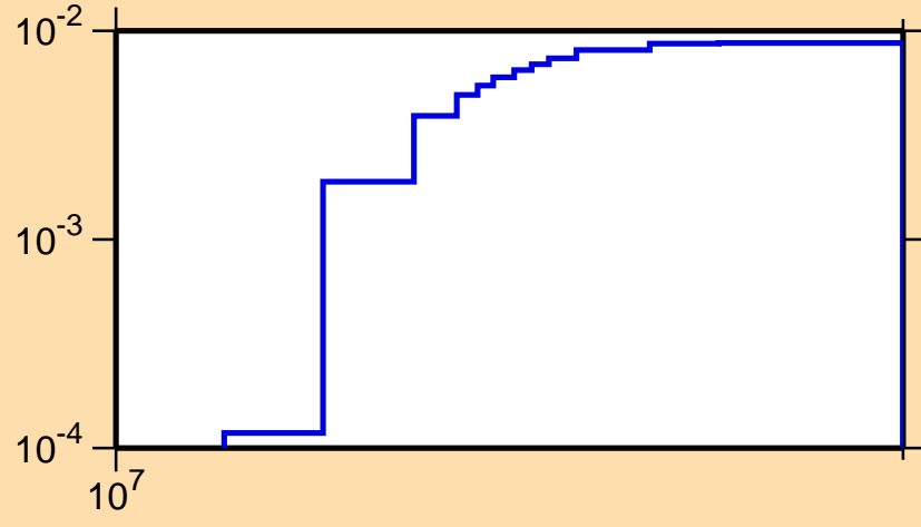
\sigma vs. E for ^{159}\text{Ta}(n,2n)
