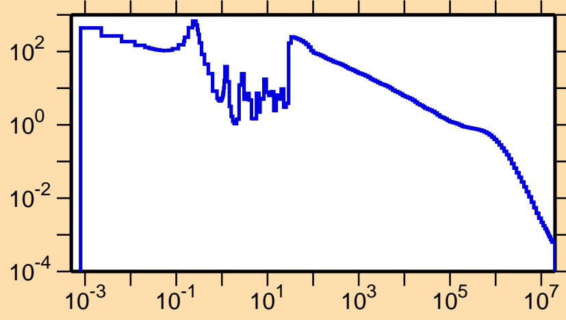
\sigma vs. E for ^{159}\text{Ta}(n,\gamma)
