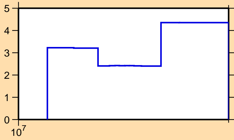
\Delta\sigma/\sigma vs. E for ^{159}\text{Ta}(n,\text{tot.})
