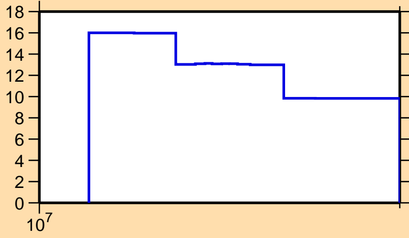
\Delta\sigma/\sigma vs. E for ^{159}\text{Ta}(n,\text{el.})
