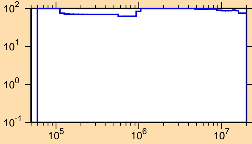
\Delta\sigma/\sigma vs. E for ^{159}\text{Ta}(n,n_1)
