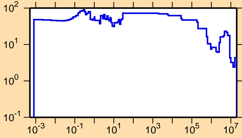
\Delta\sigma/\sigma vs. E for ^{159}\text{Ta}(n,\text{tot.})
