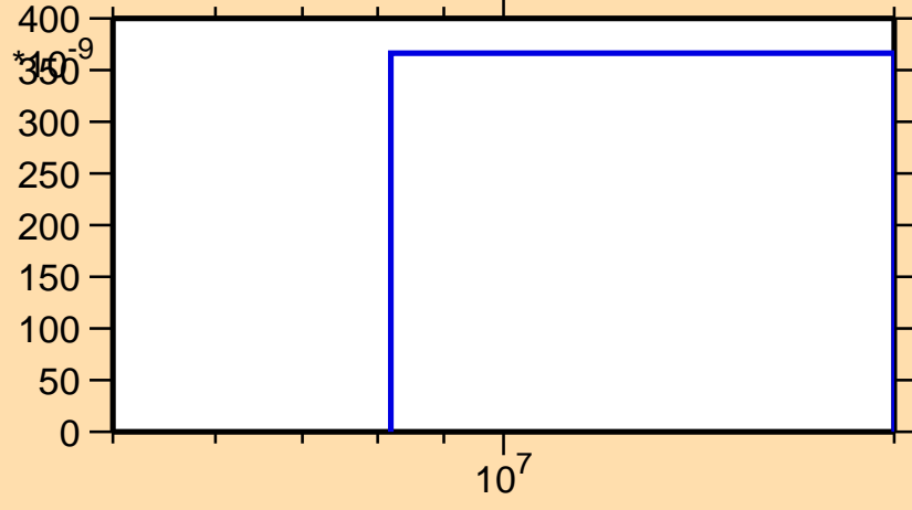
\sigma vs. E for ^{159}\text{Ta}(n,\text{nd})
