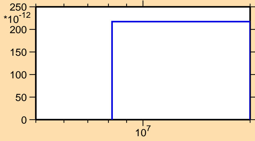
\sigma vs. E for ^{159}\text{Ta} (mt 34)
