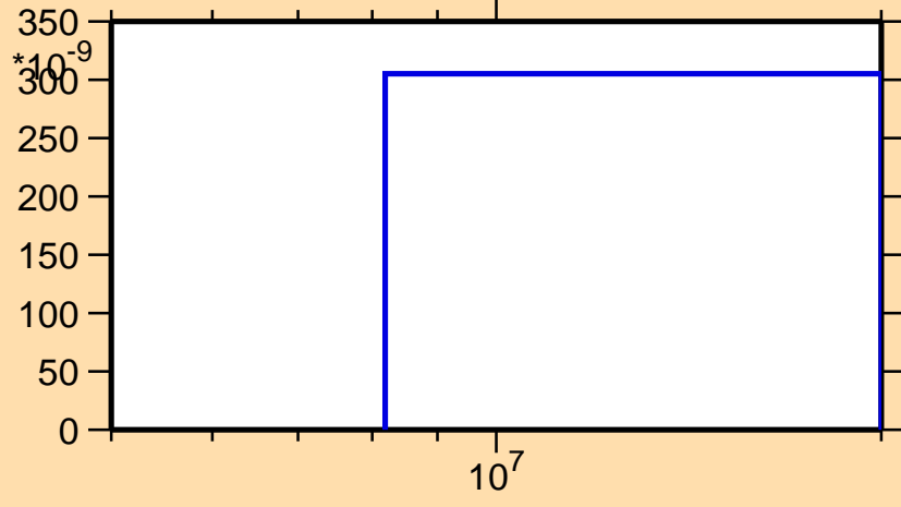
\sigma vs. E for ^{159}\text{Ta}(n,\text{pt})
