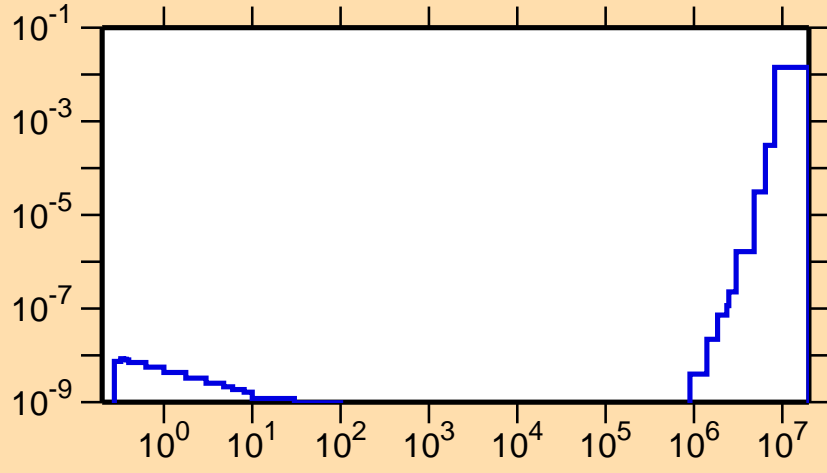
\sigma vs. E for ^{159}\text{Ta}(n,d)
