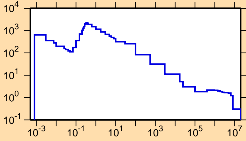
\sigma vs. E for ^{159}\text{Ta}(n,p)
