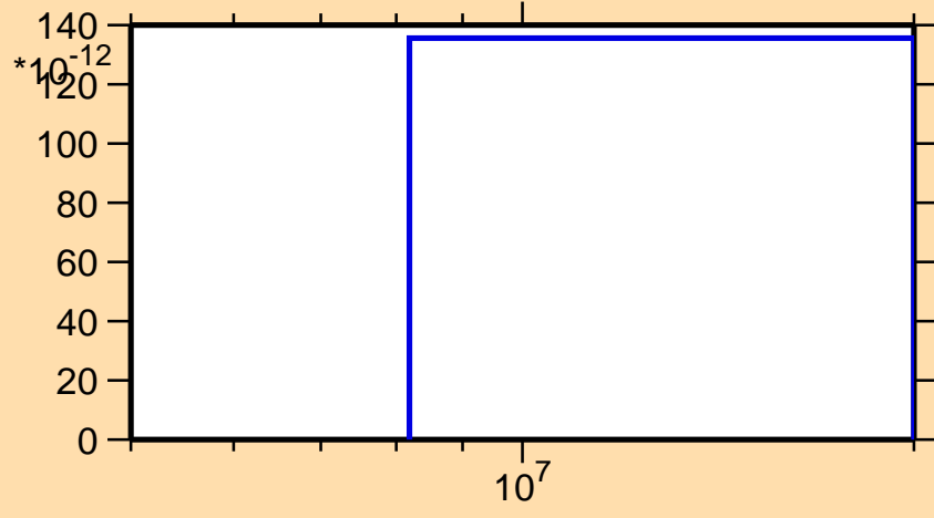
\sigma vs. E for ^{159}\text{Ta}(n,nt)
