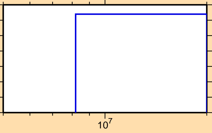
\sigma vs. E for ^{160}\text{Ta}(n,\text{pt})
