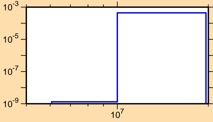
\sigma vs. E for ^{161}\text{Ta}(n,t)
