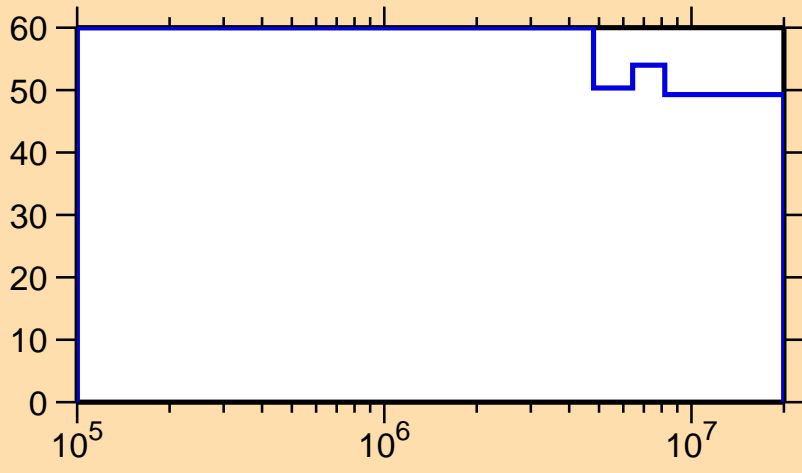
\Delta\sigma/\sigma vs. E for ^{161}\text{Ta}(n,n_1)
