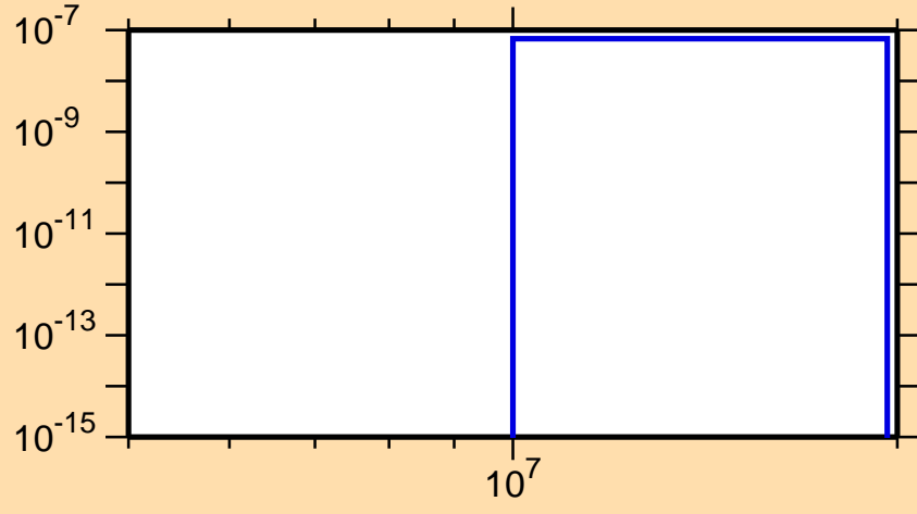
\sigma vs. E for ^{161}\text{Ta}(n,nd)
