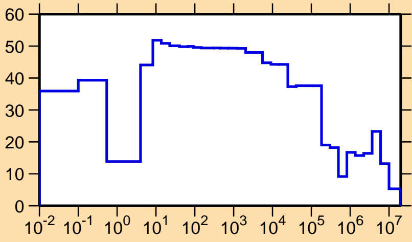
\Delta\sigma/\sigma vs. E for ^{161}\text{Ta}(n,\text{el.})
