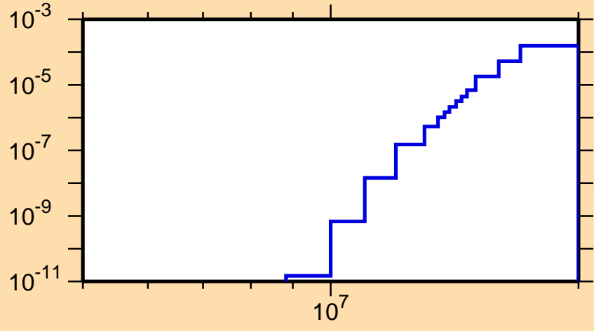
\sigma vs. E for ^{162}\text{Ta}(n,pd)
