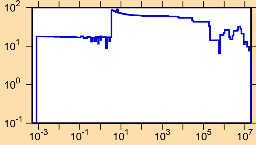
\Delta\sigma/\sigma vs. E for ^{162}\text{Ta}(n,el.)
