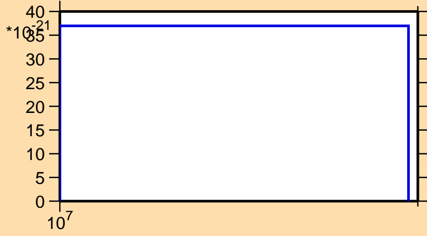
\sigma vs. E for ^{162}\text{Ta} (mt 11)
