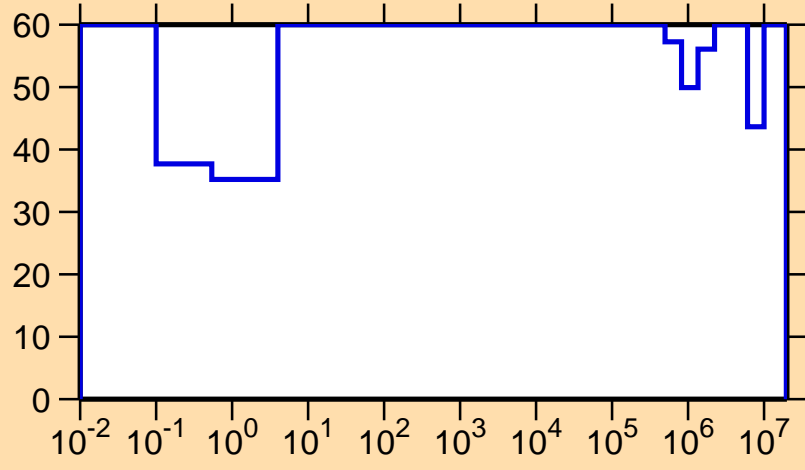
\Delta\sigma/\sigma vs. E for ^{162}\text{Ta}(n,\gamma)
