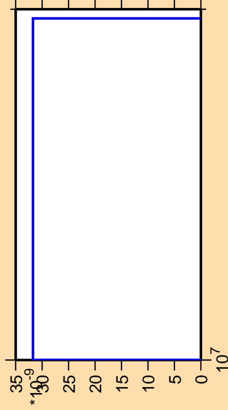
\Delta\sigma/\sigma vs. E for ^{162}\text{Ta} (mt 11)
