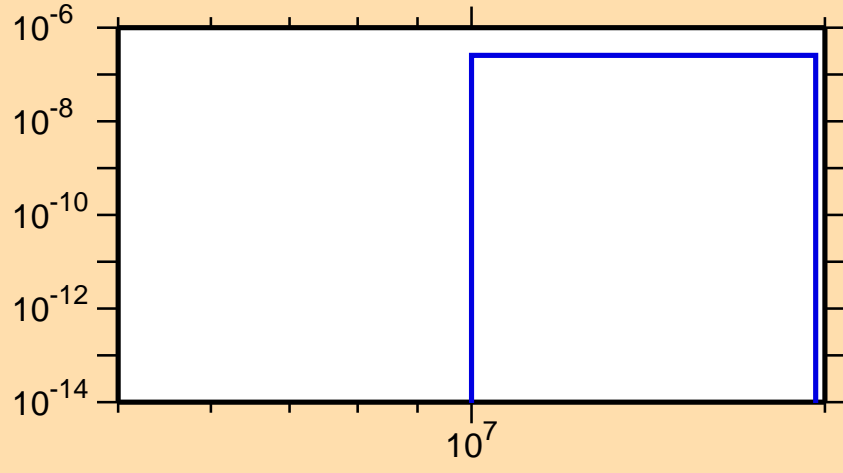
\sigma vs. E for ^{163}\text{Ta}(n,nd)
