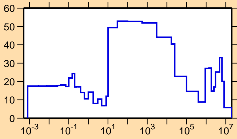
\Delta\sigma/\sigma vs. E for ^{163}\text{Ta}(n,\text{el.})
