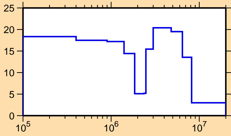
\Delta\sigma/\sigma vs. E for ^{163}\text{Ta}(n,\text{tot.})
