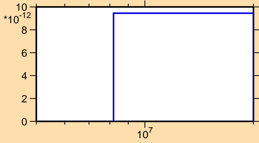
\sigma vs. E for ^{163}\text{Ta} (mt 34)
