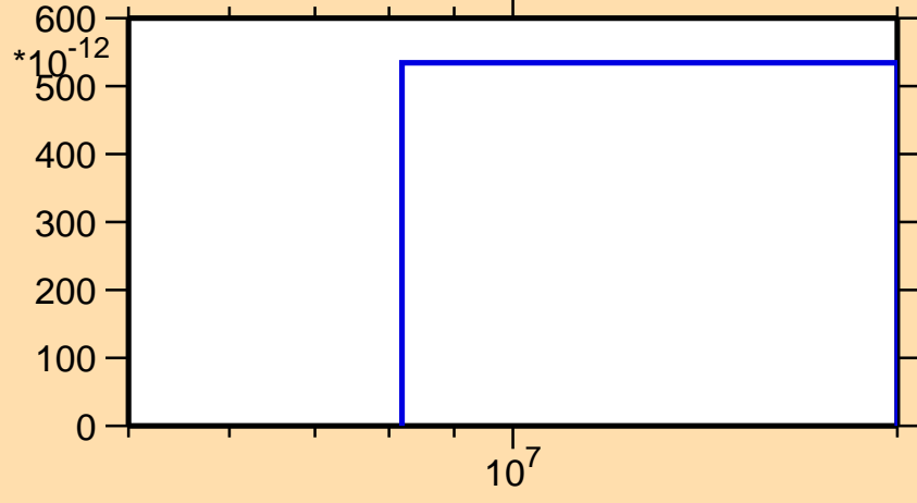
\sigma vs. E for ^{163}\text{Ta}(n,nt)
