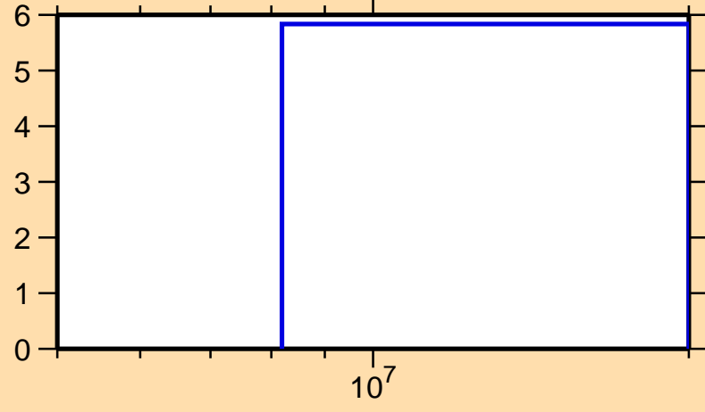
\Delta\sigma/\sigma vs. E for ^{163}\text{Ta}(n,\text{el.})
