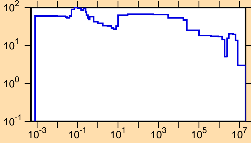
\Delta\sigma/\sigma vs. E for ^{163}\text{Ta}(n,\text{tot.})
