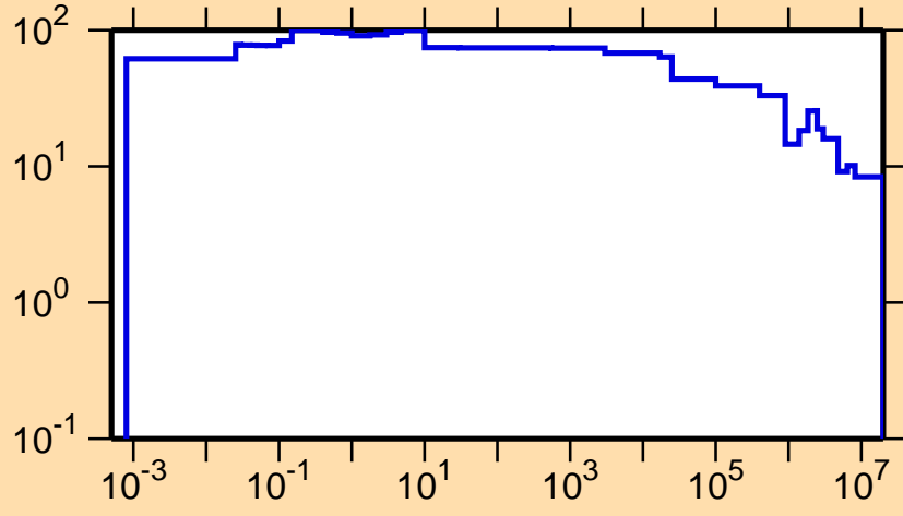
\Delta\sigma/\sigma vs. E for ^{163}\text{Ta}(n,\text{nonel.})
