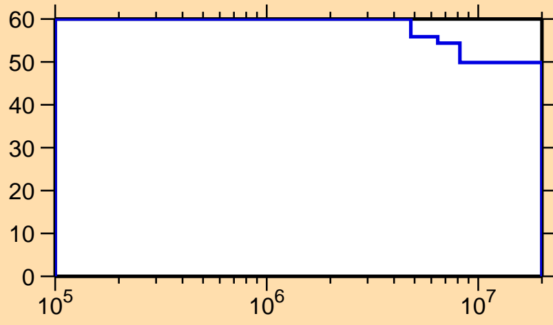
\Delta\sigma/\sigma vs. E for ^{163}\text{Ta}(n,\text{inel.})
