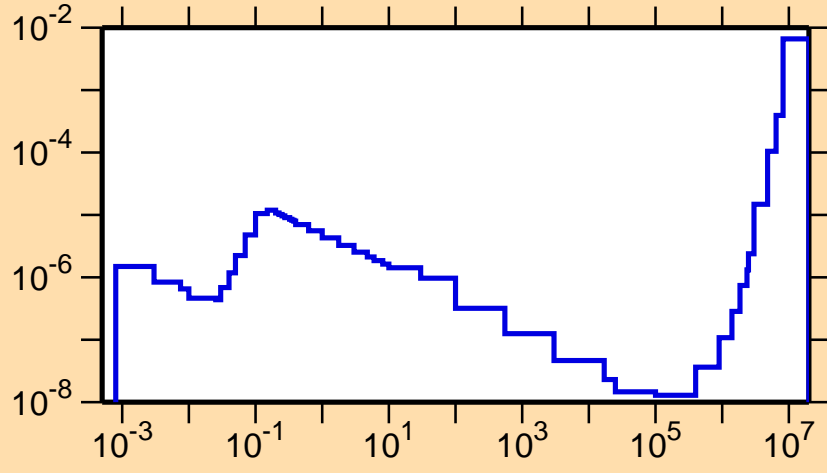
\sigma vs. E for ^{163}\text{Ta}(n,p\alpha)
