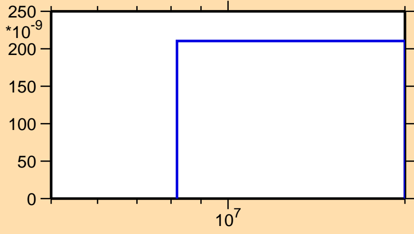
\sigma vs. E for ^{163}\text{Ta}(n,\text{nd})
