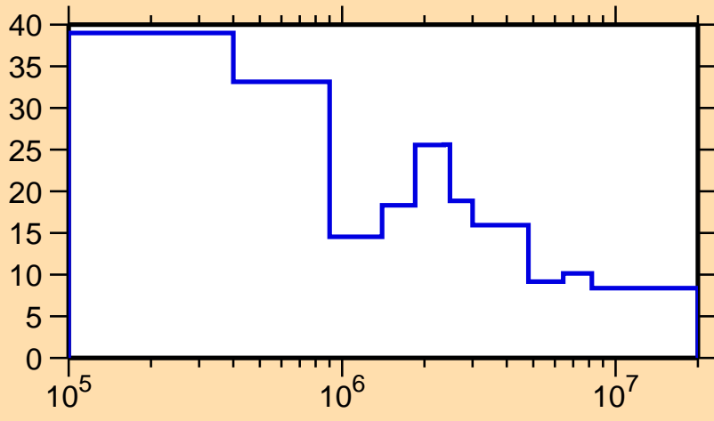
\Delta\sigma/\sigma vs. E for ^{163}\text{Ta}(n,\text{nonel.})
