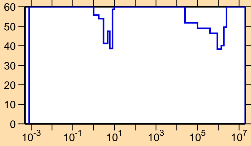
\Delta\sigma/\sigma vs. E for ^{163}\text{Ta}(n,\gamma)
