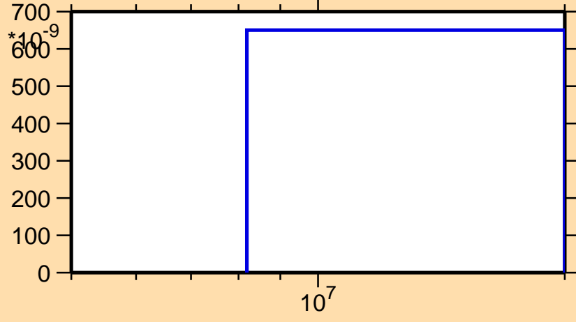
\sigma vs. E for ^{163}\text{Ta}(n,2n\alpha)
