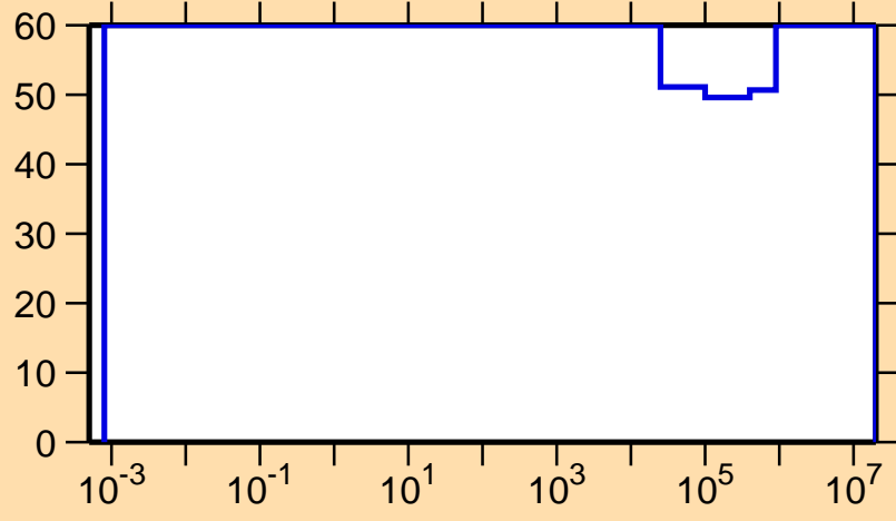
\Delta\sigma/\sigma vs. E for ^{163}\text{Ta}(n,p)
