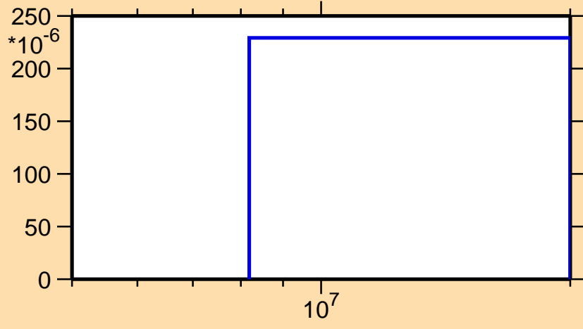
\sigma vs. E for ^{163}\text{Ta}(n,2np)
