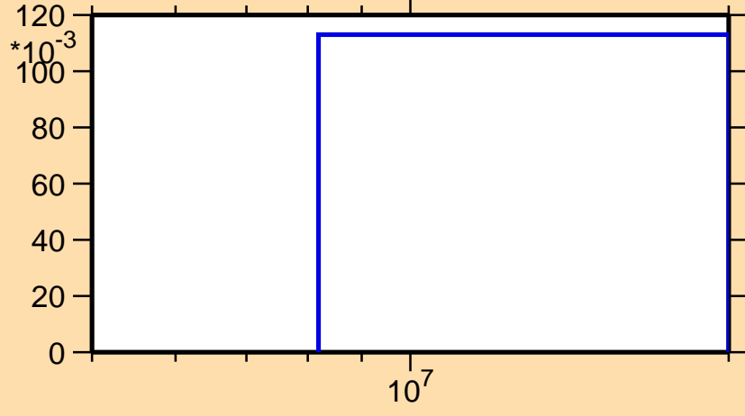
\sigma vs. E for ^{163}\text{Ta}(n,2n)
