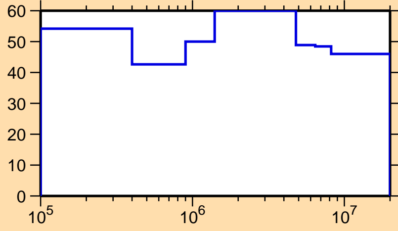
\Delta\sigma/\sigma vs. E for ^{163}\text{Ta}(n,n_1)
