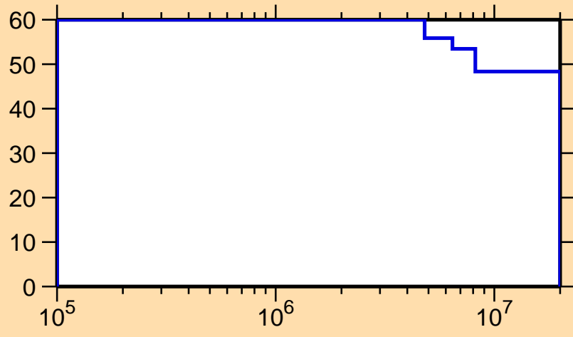
\Delta\sigma/\sigma vs. E for ^{163}\text{Ta}(n,n\text{cont.})
