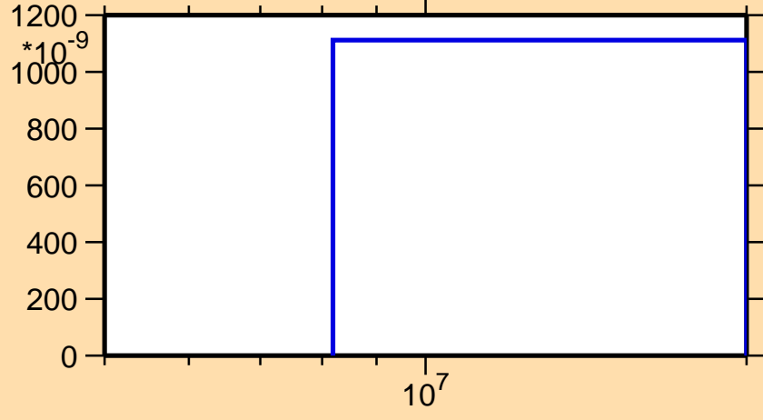
\sigma vs. E for ^{163}\text{Ta}(n,pd)
