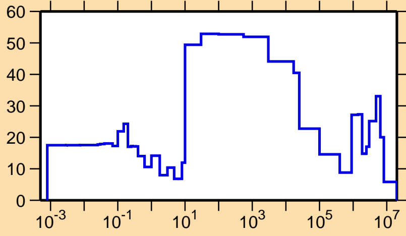
\Delta\sigma/\sigma vs. E for ^{163}\text{Ta}(n,\text{el.})
