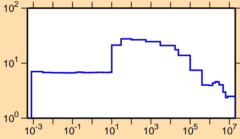
\sigma vs. E for ^{163}\text{Ta}(n,\text{el.})
