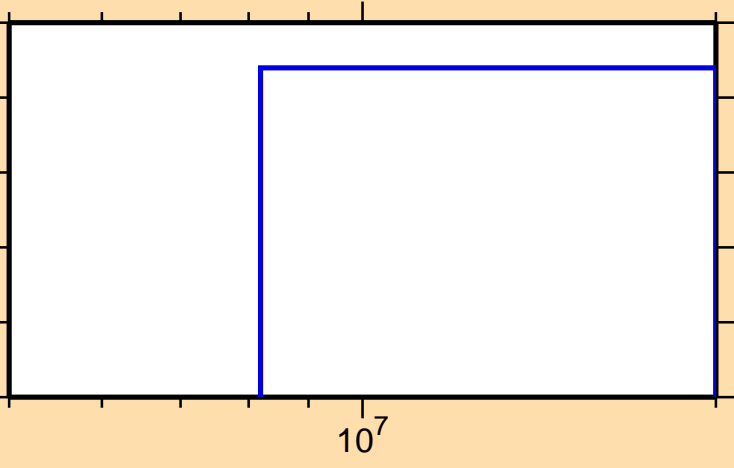
\sigma vs. E for ^{163}\text{Ta}(n,\text{pt})
