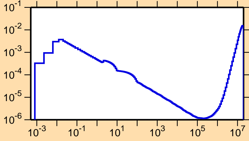
\sigma vs. E for ^{164}\text{Ta}(n,p\alpha)
