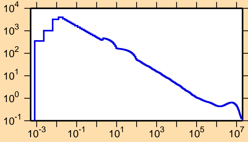
\sigma vs. E for ^{164}\text{Ta}(n,p)
