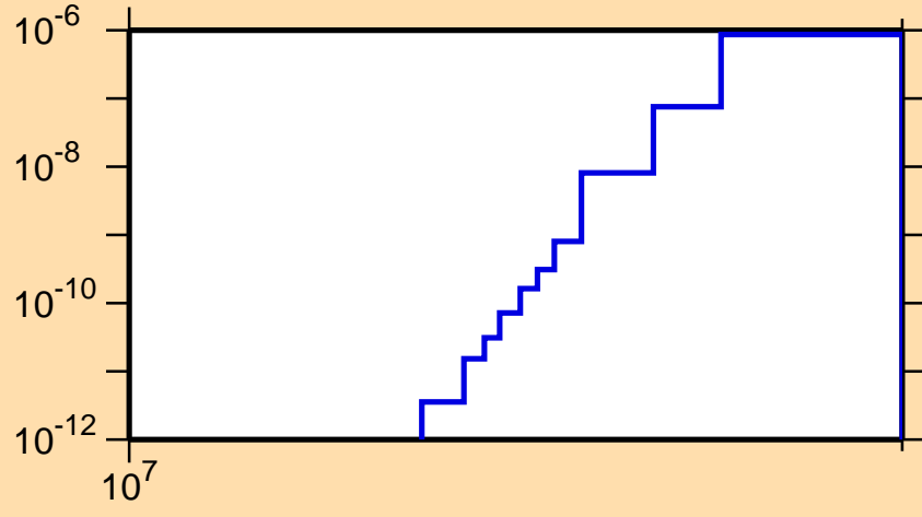
\sigma vs. E for ^{164}\text{Ta}(n,\text{pt})
