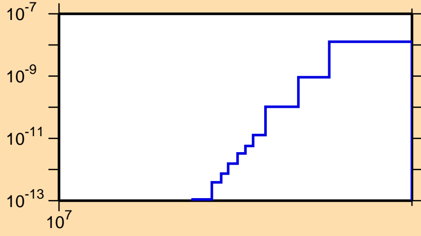
\sigma vs. E for ^{164}\text{Ta} (mt 34)
