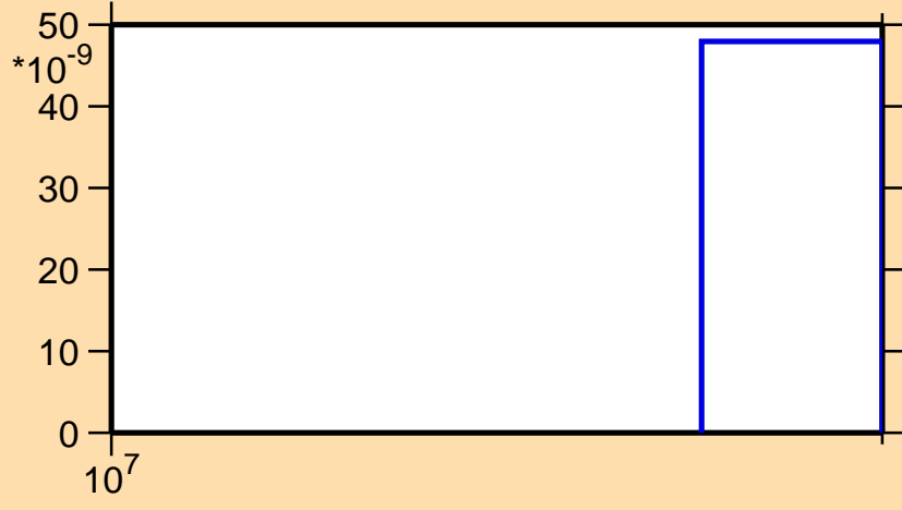
\sigma vs. E for ^{164}\text{Ta}(n,3n)
