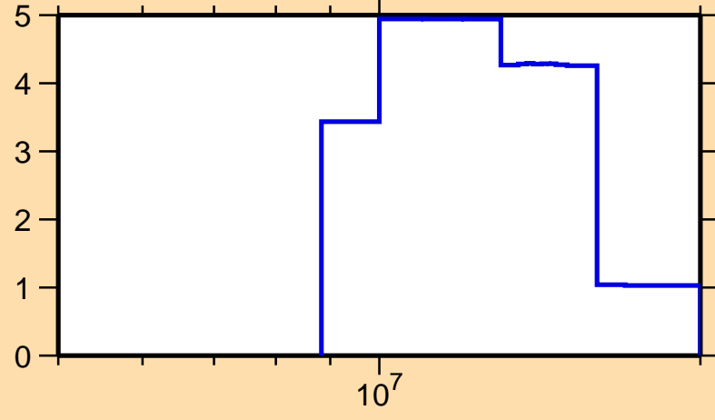
\Delta\sigma/\sigma vs. E for ^{164}\text{Ta}(n,\text{tot.})
