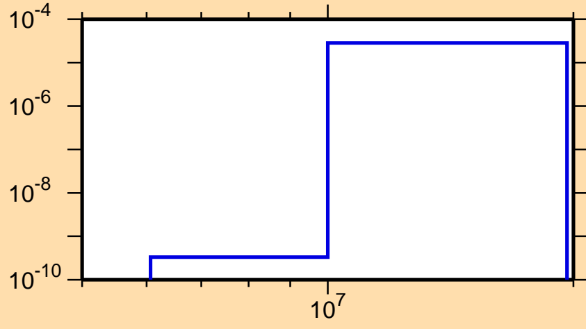
\sigma vs. E for ^{164}\text{Ta} (mt 45)
