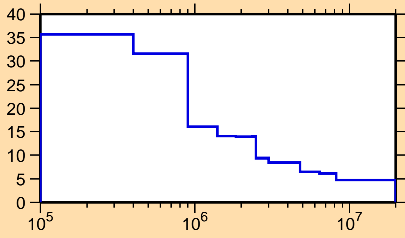
\Delta\sigma/\sigma vs. E for ^{164}\text{Ta}(n,\text{nonel.})
