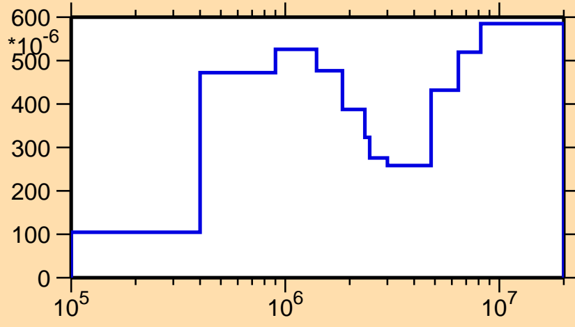
\sigma vs. E for ^{164}\text{Ta}(n,n_3)
