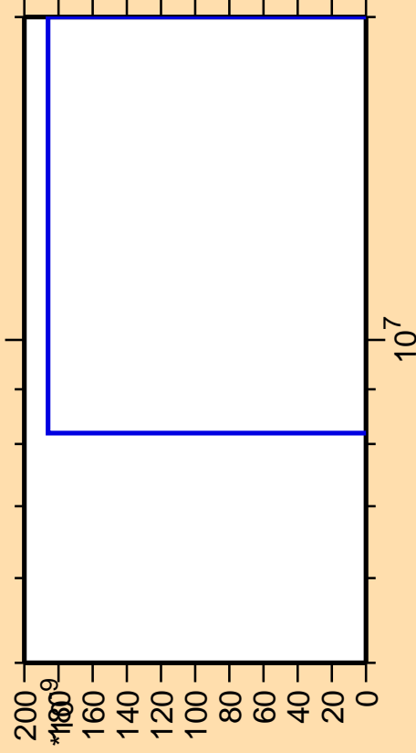
\Delta\sigma/\sigma vs. E for ^{164}\text{Ta} (mt 11)
