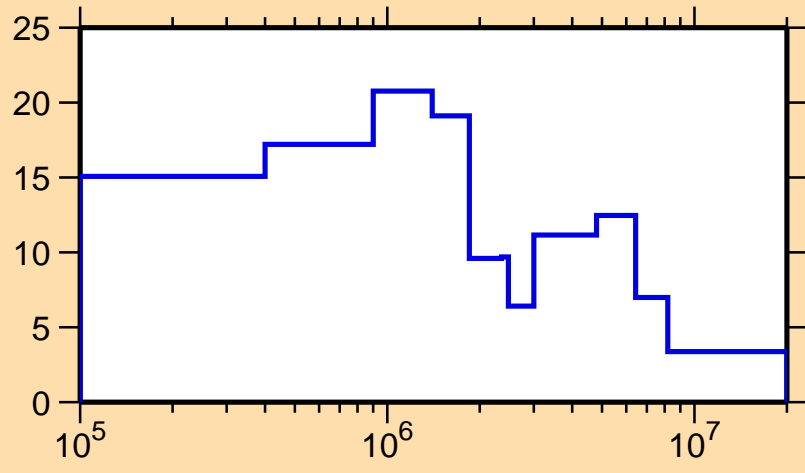
\Delta\sigma/\sigma vs. E for ^{164}\text{Ta}(n,\text{tot.})
