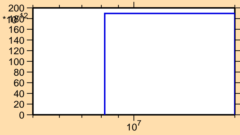
\sigma vs. E for ^{164}\text{Ta}(n,nt)
