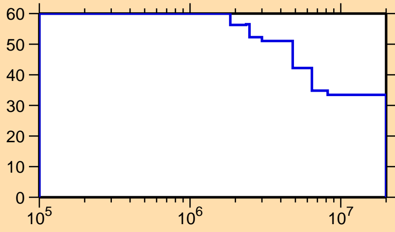
\Delta\sigma/\sigma vs. E for ^{164}\text{Ta}(n,n_1)
