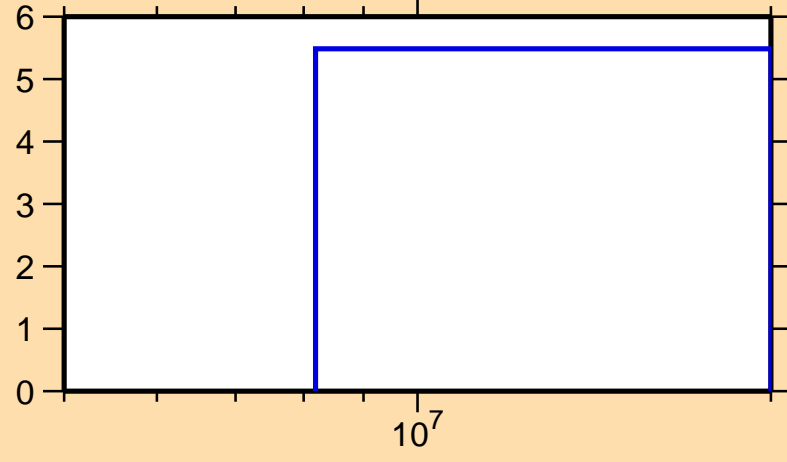
\Delta\sigma/\sigma vs. E for ^{164}\text{Ta}(n,\text{el.})
