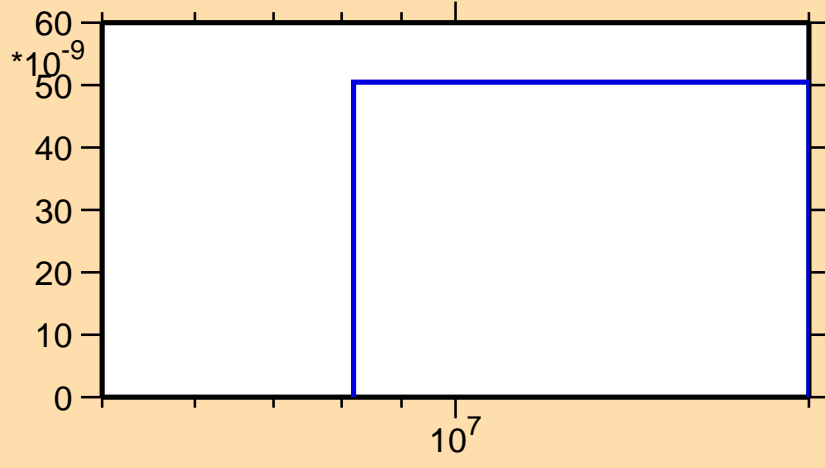
\sigma vs. E for ^{164}\text{Ta}(\text{mt117})
