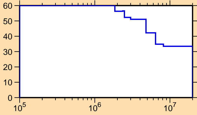
\Delta\sigma/\sigma vs. E for ^{164}\text{Ta}(n,n_1)
