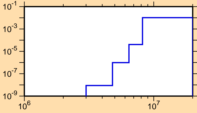
\sigma vs. E for ^{164}\text{Ta}(n,d)
