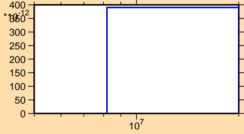
\sigma vs. E for ^{164}\text{Ta}(n,3n)
