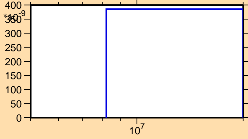
\sigma vs. E for ^{164}\text{Ta}(n,pd)
