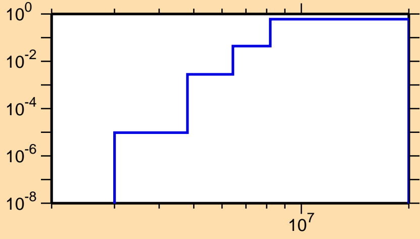
\sigma vs. E for ^{164}\text{Ta}(n,np)
