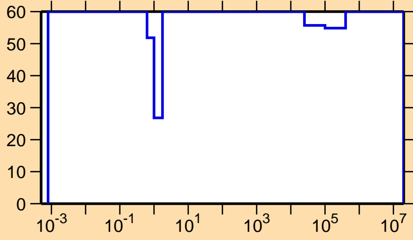
\Delta\sigma/\sigma vs. E for ^{164}\text{Ta}(n,\gamma)
