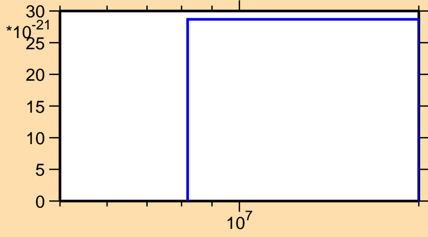
\sigma vs. E for ^{164}\text{Ta} (mt 11)
