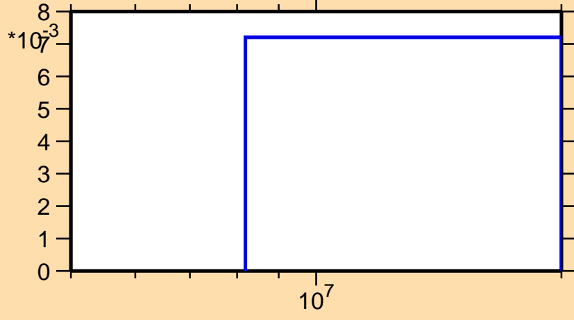
\sigma vs. E for ^{164}\text{Ta}(n,2np)
