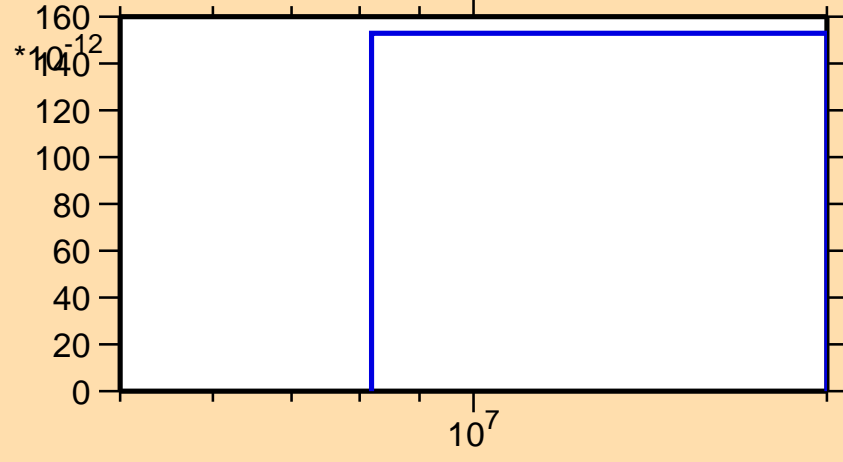
\sigma vs. E for ^{164}\text{Ta} (mt 34)
