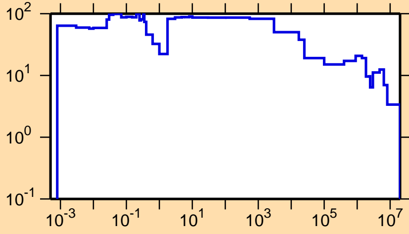
\Delta\sigma/\sigma vs. E for ^{164}\text{Ta}(n,\text{tot.})
