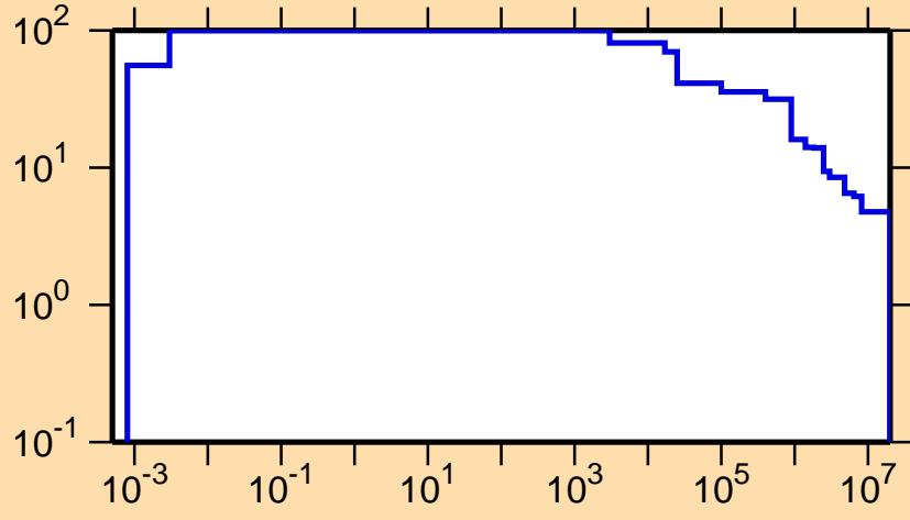
\Delta\sigma/\sigma vs. E for ^{164}\text{Ta}(n,\text{nonel.})
