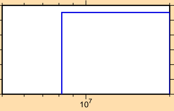
\sigma vs. E for ^{164}\text{Ta}(n,\text{pt})
