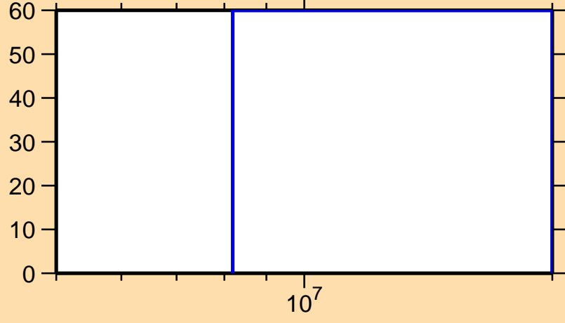
\Delta\sigma/\sigma vs. E for ^{164}\text{Ta}(n,\text{inel.})
