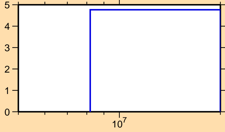
\Delta\sigma/\sigma vs. E for ^{164}\text{Ta}(n,\text{nonel.})
