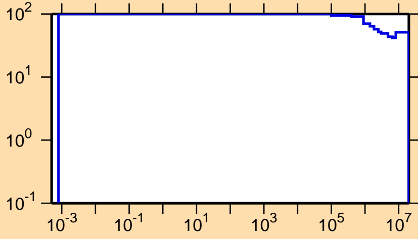
\Delta\sigma/\sigma vs. E for ^{164}\text{Ta}(n,p)
