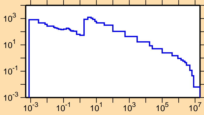
\sigma vs. E for ^{164}\text{Ta}(n,\gamma)
