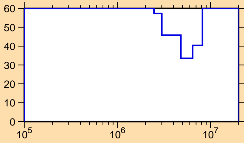
\Delta\sigma/\sigma vs. E for ^{164}\text{Ta}(n,\text{inel.})
