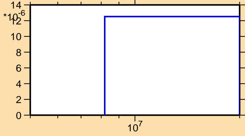
\sigma vs. E for ^{164}\text{Ta}(n,2n\alpha)
