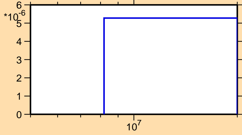
\sigma vs. E for ^{164}\text{Ta}(n,\text{nd})
