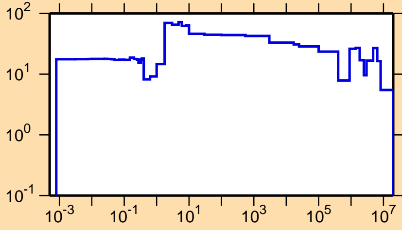
\Delta\sigma/\sigma vs. E for ^{164}\text{Ta}(n,\text{el.})
