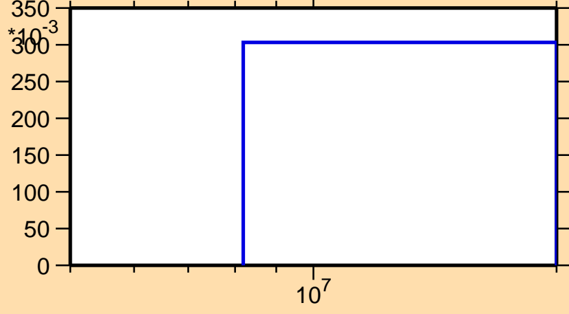
\sigma vs. E for ^{164}\text{Ta}(n,2n)
