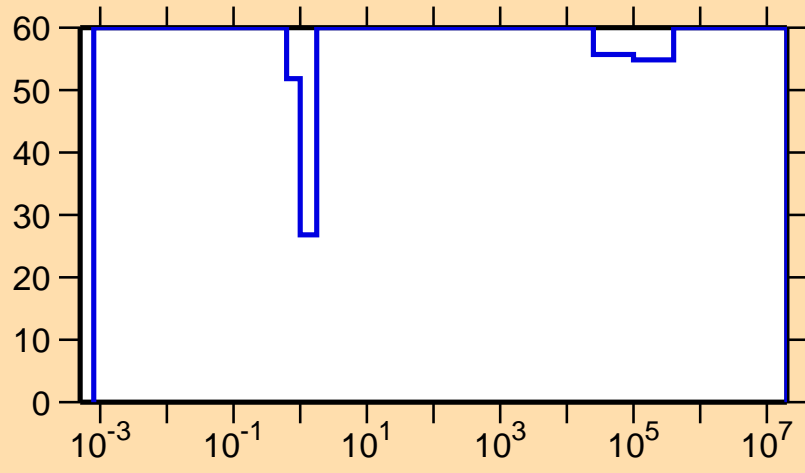
\Delta\sigma/\sigma vs. E for ^{164}\text{Ta}(n,\gamma)
