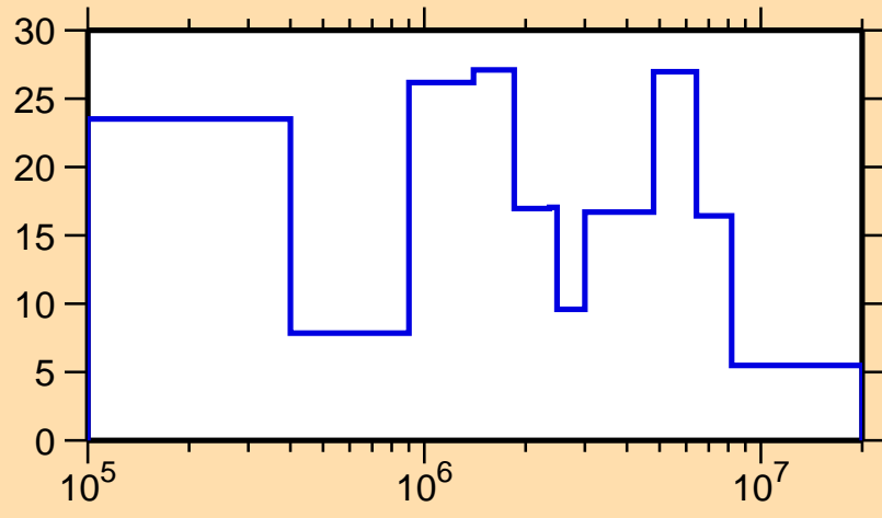
\Delta\sigma/\sigma vs. E for ^{164}\text{Ta}(n,\text{el.})
