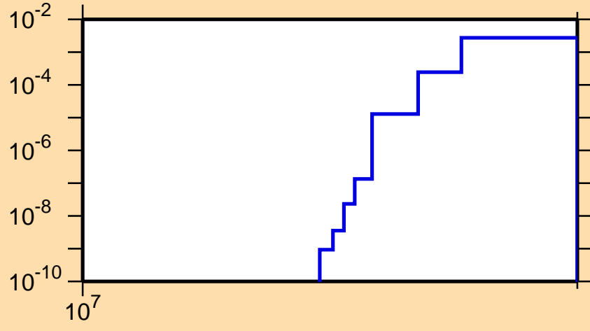
\sigma vs. E for ^{165}\text{Ta}(n,2np)
