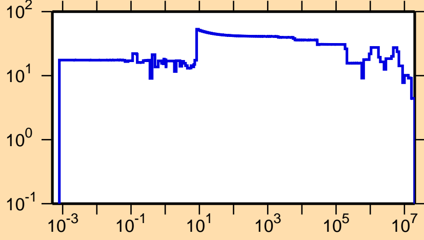
\Delta\sigma/\sigma vs. E for ^{165}\text{Ta}(n,\text{el.})
