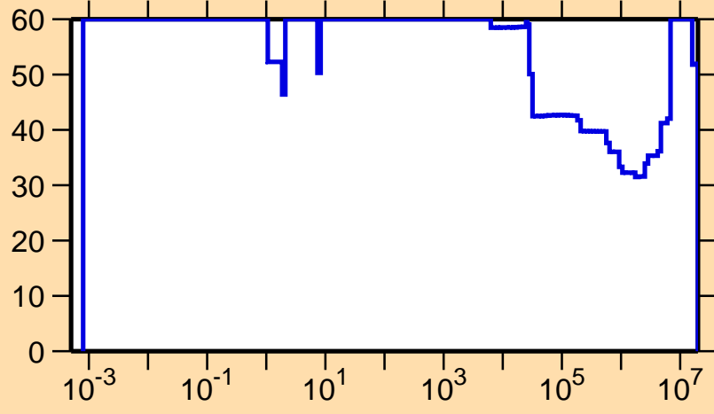
\Delta\sigma/\sigma vs. E for ^{165}\text{Ta}(n,\gamma)
