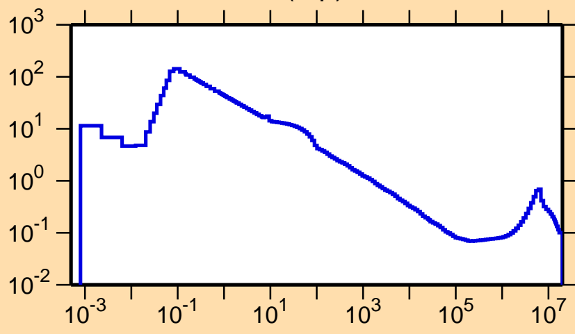
\sigma vs. E for ^{165}\text{Ta}(n,p)
