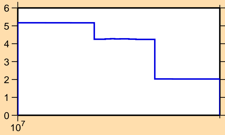
\Delta\sigma/\sigma vs. E for ^{165}\text{Ta}(n,\text{tot.})
