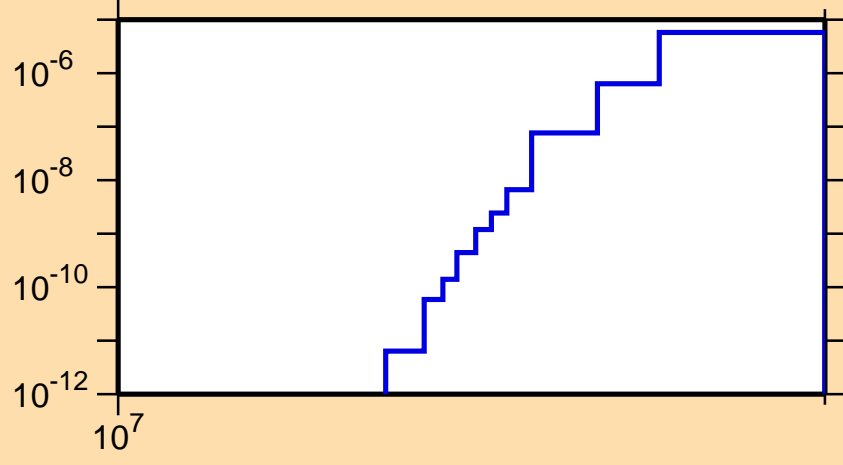
\sigma vs. E for ^{165}\text{Ta}(n,\text{nd})
