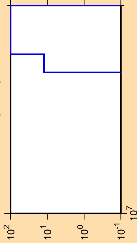
\Delta\sigma/\sigma vs. E for ^{165}\text{Ta} (mt 34)
