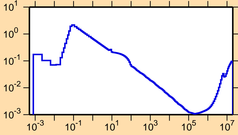
\sigma vs. E for ^{165}\text{Ta}(n,\alpha)
