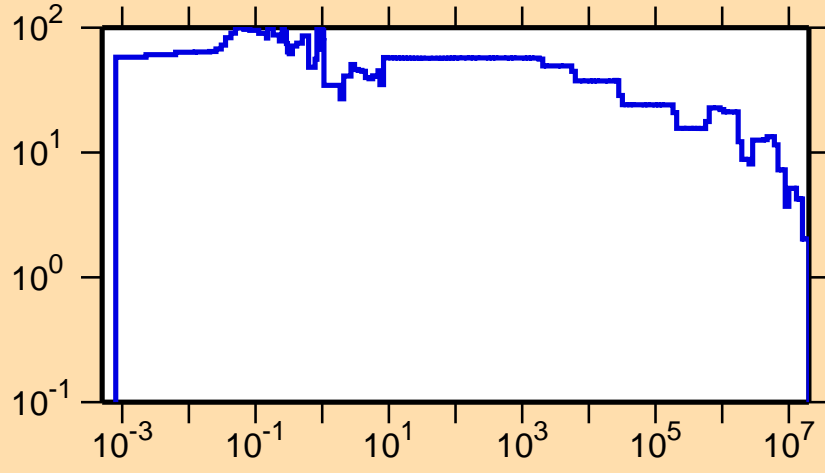
\Delta\sigma/\sigma vs. E for ^{165}\text{Ta}(n,\text{tot.})
