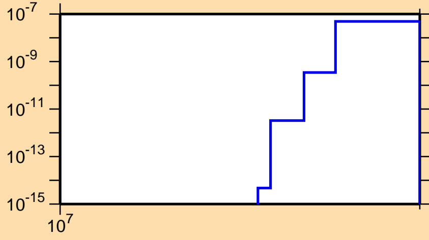
\sigma vs. E for ^{165}\text{Ta}(n,nt)
