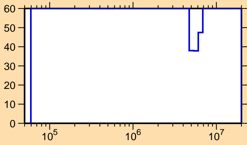
\Delta\sigma/\sigma vs. E for ^{165}\text{Ta}(n,\text{inel.})
