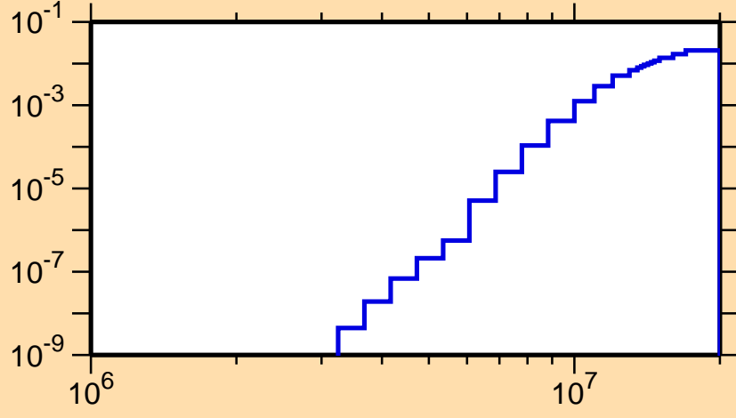
\sigma vs. E for ^{165}\text{Ta}(n,d)
