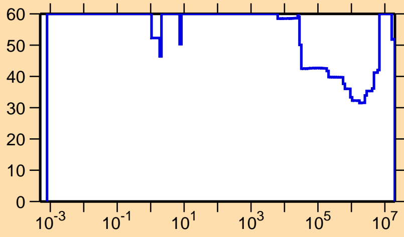
\Delta\sigma/\sigma vs. E for ^{165}\text{Ta}(n,\gamma)
