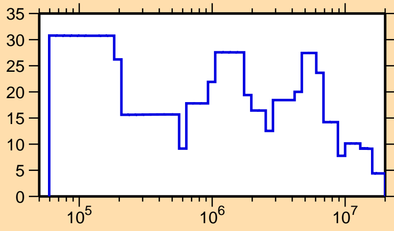
\Delta\sigma/\sigma vs. E for ^{165}\text{Ta}(n,\text{el.})
