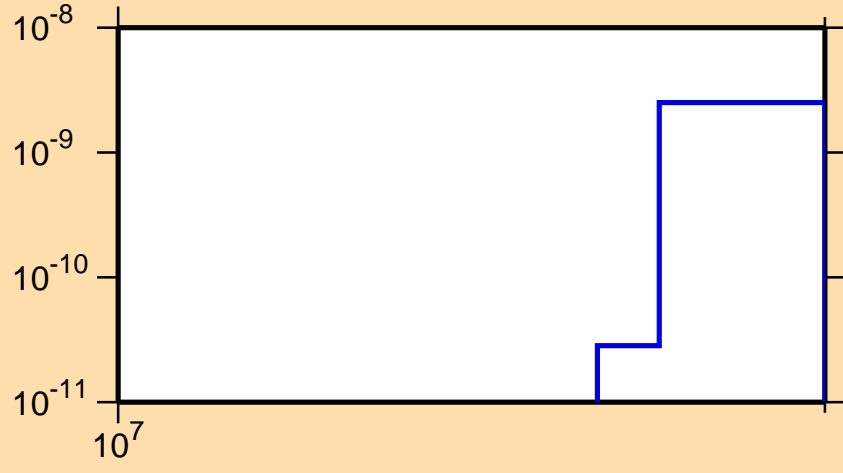
\sigma vs. E for ^{165}\text{Ta}(n,\text{pt})
