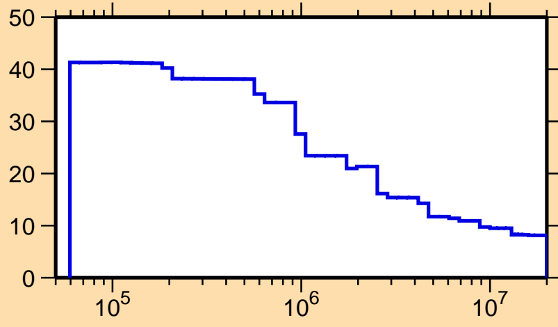
\Delta\sigma/\sigma vs. E for ^{165}\text{Ta}(n,\text{nonel.})
