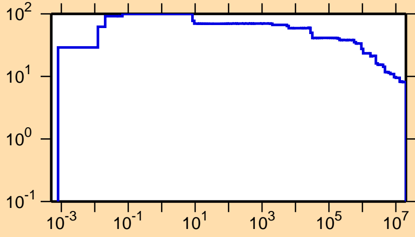
\Delta\sigma/\sigma vs. E for ^{165}\text{Ta}(n,\text{nonel.})
