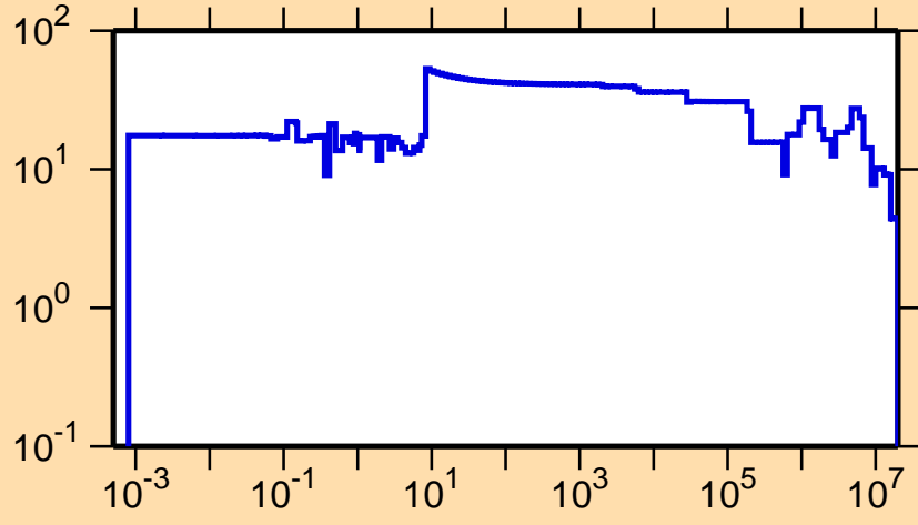
\Delta\sigma/\sigma vs. E for ^{165}\text{Ta}(n,el.)
