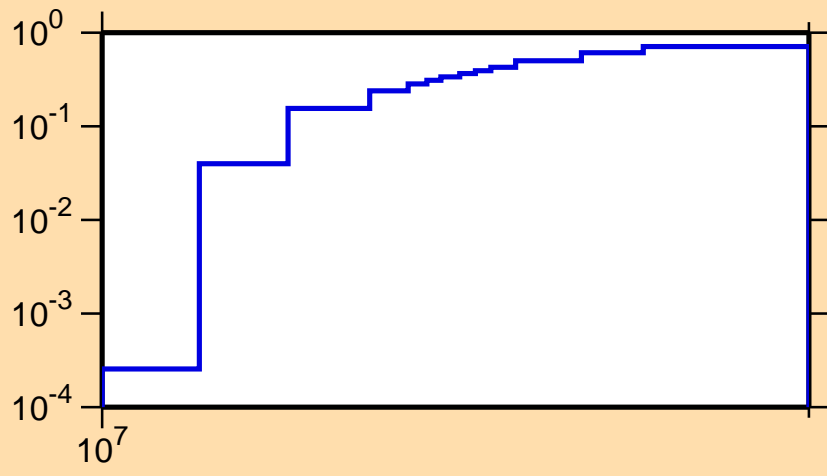
\sigma vs. E for ^{165}\text{Ta}(n,2n)
