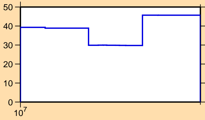
\Delta\sigma/\sigma vs. E for ^{165}\text{Ta}(n,2n)
