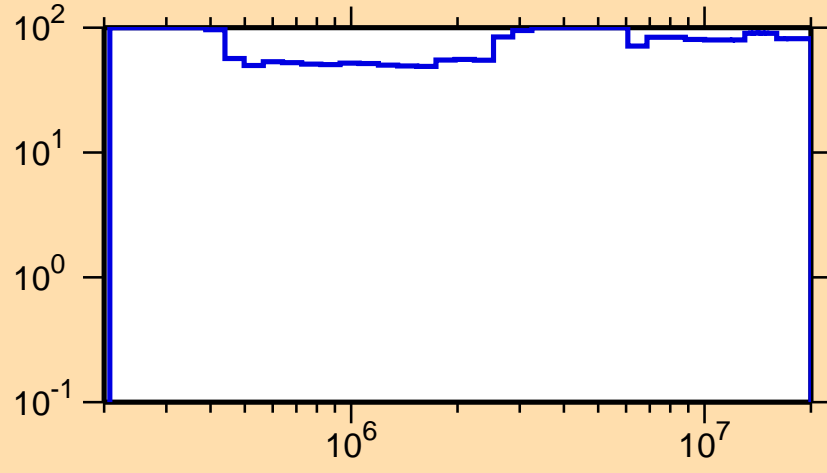
\Delta\sigma/\sigma vs. E for ^{165}\text{Ta}(n,n\text{cont.})
