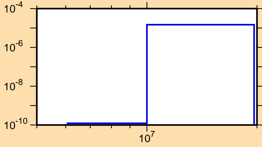
\sigma vs. E for ^{165}\text{Ta} (mt 45)
