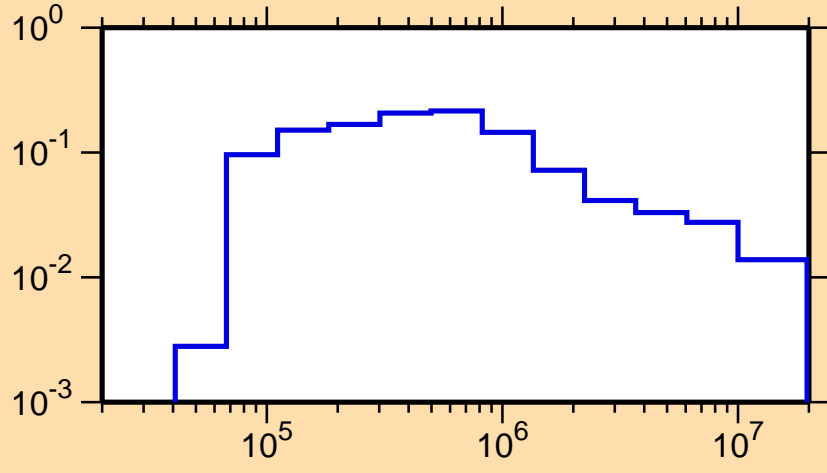
\sigma vs. E for ^{165}\text{Ta}(n,n_1)
