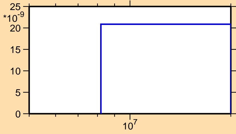
\sigma vs. E for ^{165}\text{Ta}(\text{mt117})
