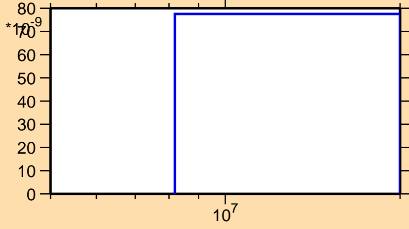
\sigma vs. E for ^{165}\text{Ta}(n,pd)
