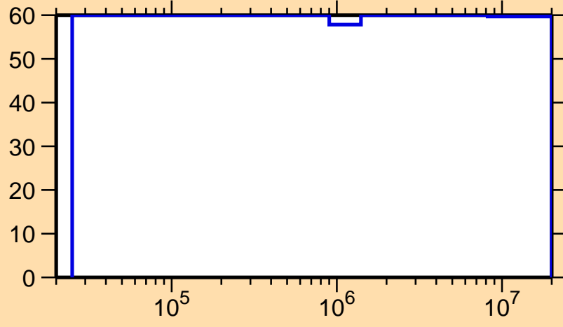
\Delta\sigma/\sigma vs. E for ^{165}\text{Ta}(n,n_1)
