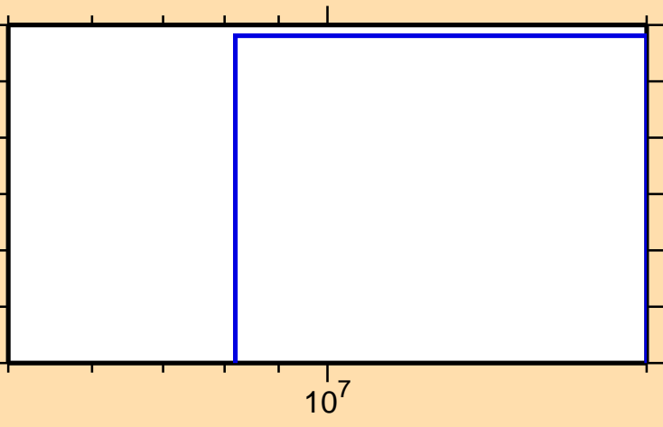
\sigma vs. E for ^{165}\text{Ta}(n,3n)
