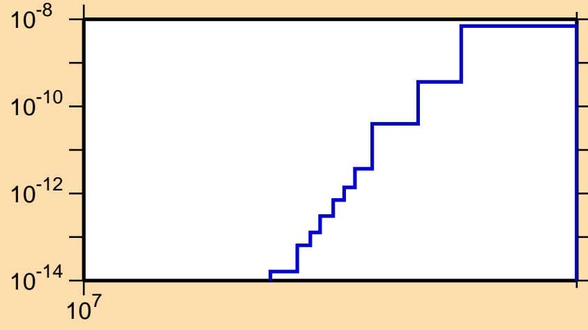
\sigma vs. E for ^{166}\text{Ta} (mt 34)
