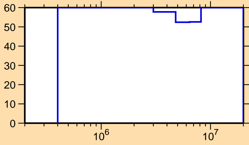
\Delta\sigma/\sigma vs. E for ^{166}\text{Ta}(n,n\text{cont.})
