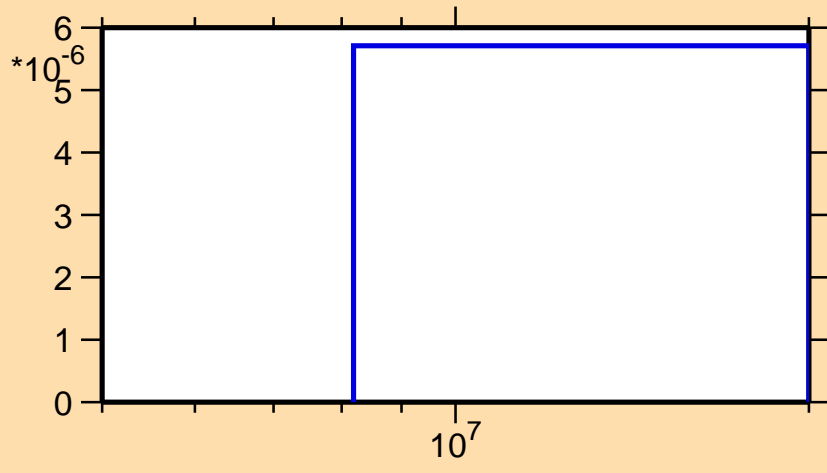
\sigma vs. E for ^{166}\text{Ta}(n,\text{nd})
