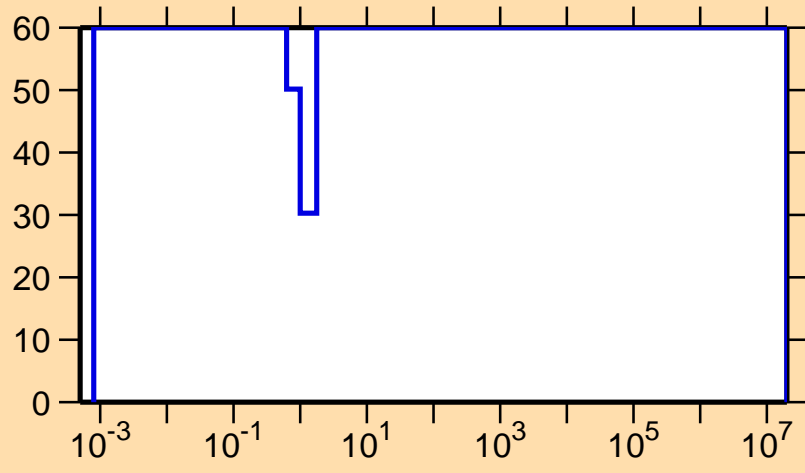
\Delta\sigma/\sigma vs. E for ^{166}\text{Ta}(n,\gamma)
