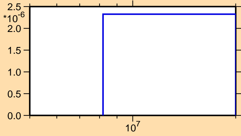
\sigma vs. E for ^{166}\text{Ta} (mt 45)
