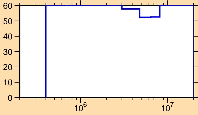
\Delta\sigma/\sigma vs. E for ^{166}\text{Ta}(n,n\text{cont.})
