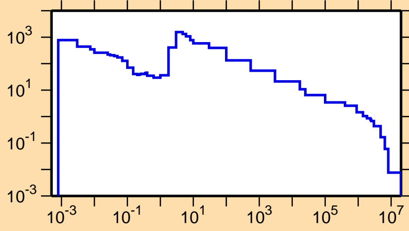
\sigma vs. E for ^{166}\text{Ta}(n,\gamma)
