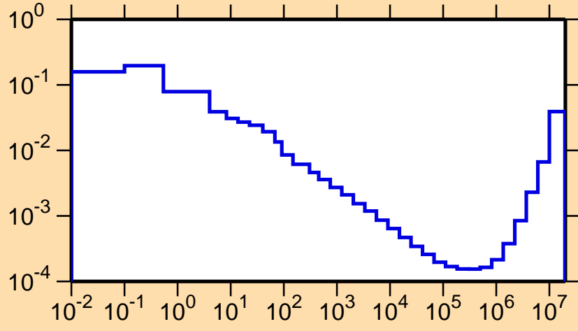
\sigma vs. E for ^{167}\text{Ta}(n,\alpha)
