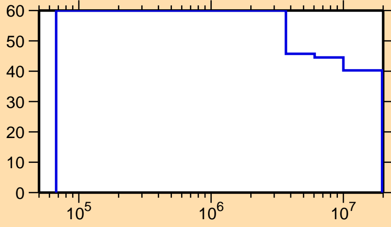
\Delta\sigma/\sigma vs. E for ^{167}\text{Ta}(n,n_1)
