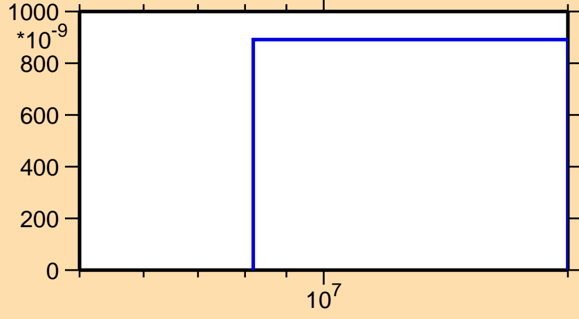
\sigma vs. E for ^{167}\text{Ta} (mt 45)
