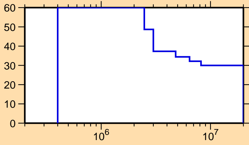
\Delta\sigma/\sigma vs. E for ^{167}\text{Ta}(n,n\text{cont.})
