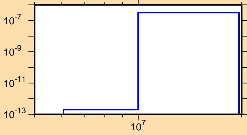
\sigma vs. E for ^{168}\text{Ta} (mt 45)
