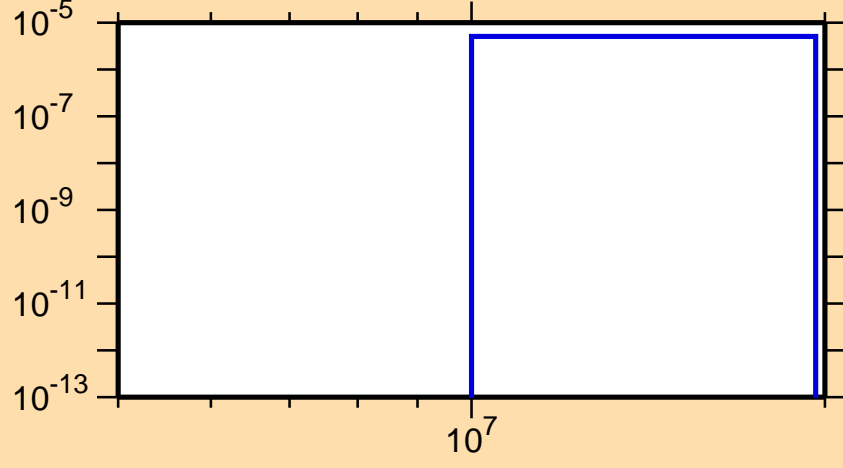
\sigma vs. E for ^{168}\text{Ta}(n,nd)
