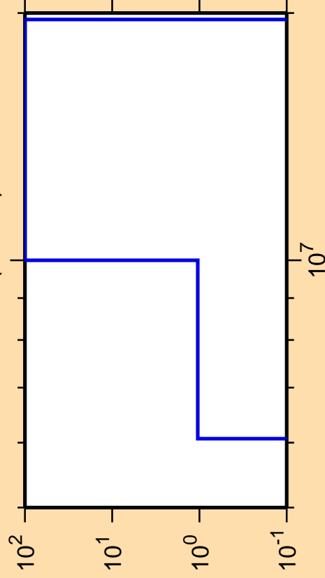
\Delta\sigma/\sigma vs. E for ^{168}\text{Ta} (mt 45)
