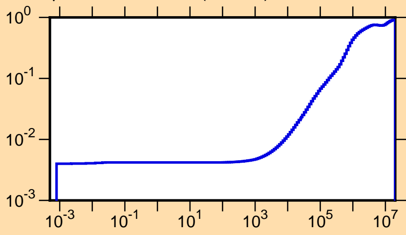
\mu vs. E for ^{169}\text{Ta}(\text{mt251})
