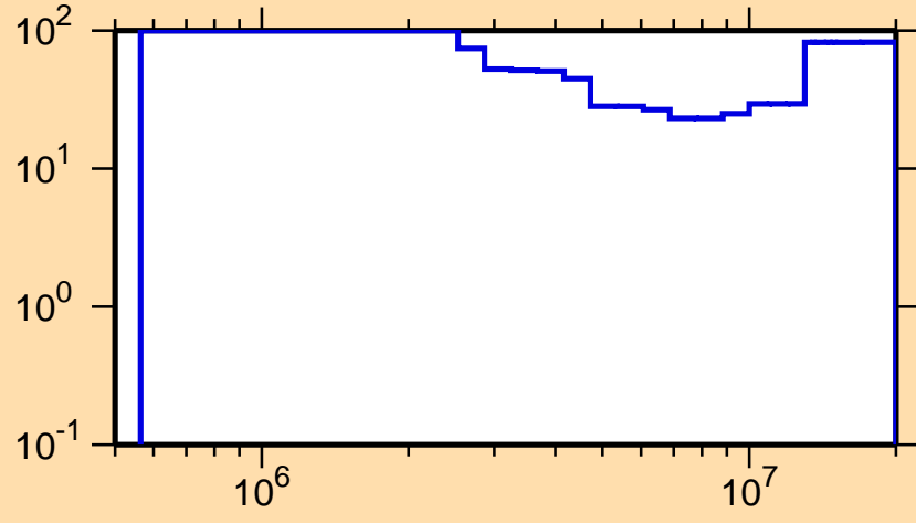
\Delta\sigma/\sigma vs. E for ^{169}\text{Ta}(n,n\text{cont.})
