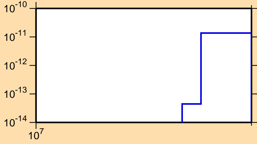
\sigma vs. E for ^{169}\text{Ta}(n,\text{pt})
