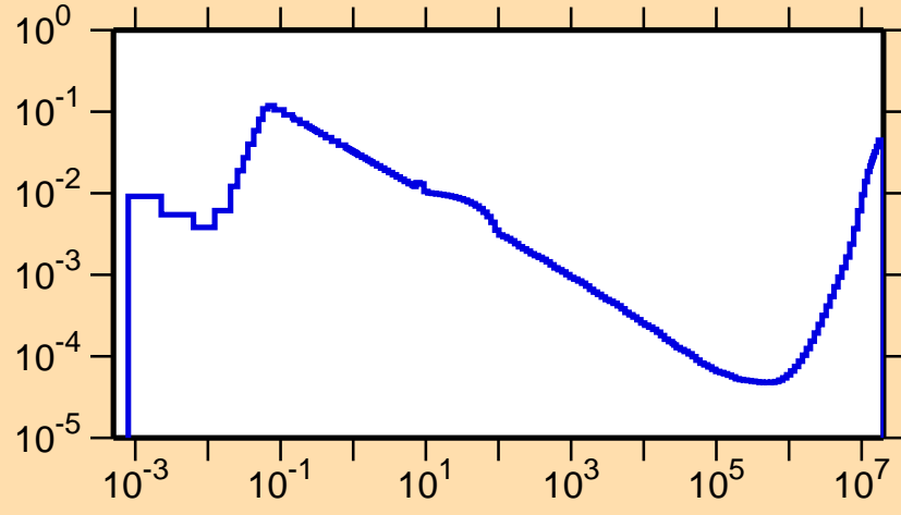
\sigma vs. E for ^{169}\text{Ta}(n,\alpha)
