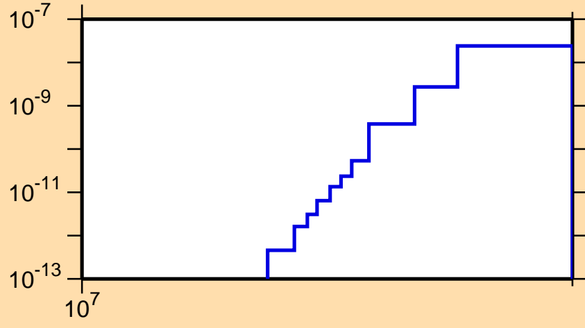
\sigma vs. E for ^{169}\text{Ta}(n,pd)
