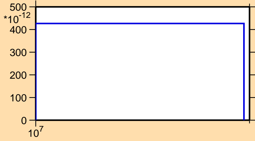
\sigma vs. E for ^{169}\text{Ta}(n,\text{pd})
