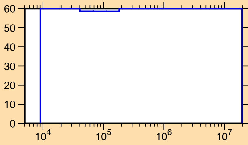
\Delta\sigma/\sigma vs. E for ^{169}\text{Ta}(n,n_1)
