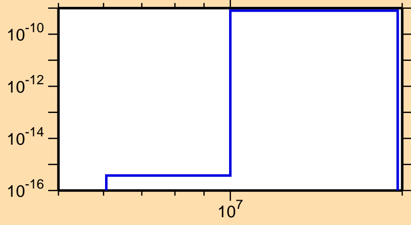
\sigma vs. E for ^{169}\text{Ta}(\text{mt117})
