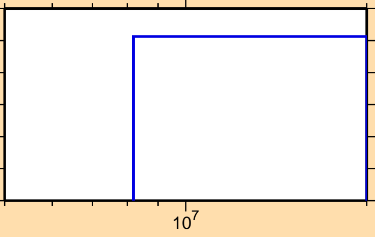
\sigma vs. E for ^{169}\text{Ta}(n,nt)
