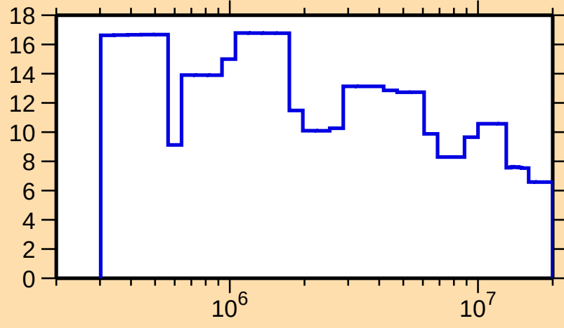
\Delta\sigma/\sigma vs. E for ^{170}\text{Ta}(n,\text{el.})
