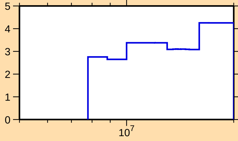
\Delta\sigma/\sigma vs. E for ^{170}\text{Ta}(n,\text{tot.})
