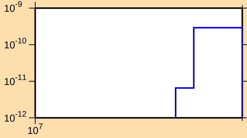
\sigma vs. E for ^{170}\text{Ta} (mt 34)
