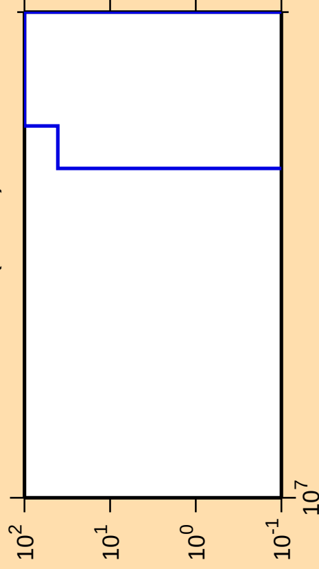
\Delta\sigma/\sigma vs. E for ^{170}\text{Ta} (mt 34)
