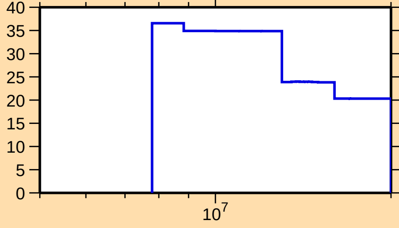
\Delta\sigma/\sigma vs. E for ^{170}\text{Ta}(n,2n)
