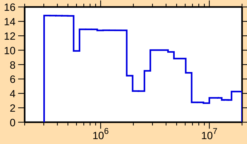
\Delta\sigma/\sigma vs. E for ^{170}\text{Ta}(n,\text{tot.})
