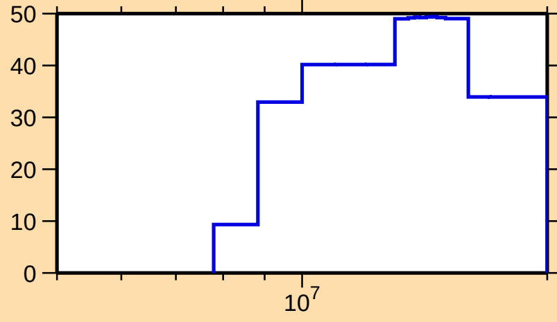
\Delta\sigma/\sigma vs. E for ^{170}\text{Ta}(n,\text{inel.})
