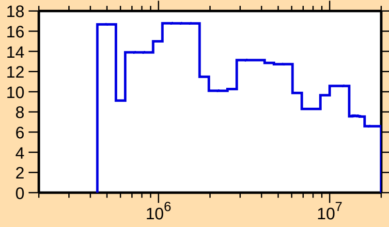
\Delta\sigma/\sigma vs. E for ^{170}\text{Ta}(n,\text{el.})
