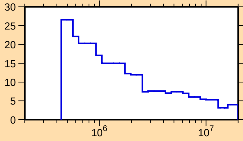
\Delta\sigma/\sigma vs. E for ^{170}\text{Ta}(n,n\text{onel.})
