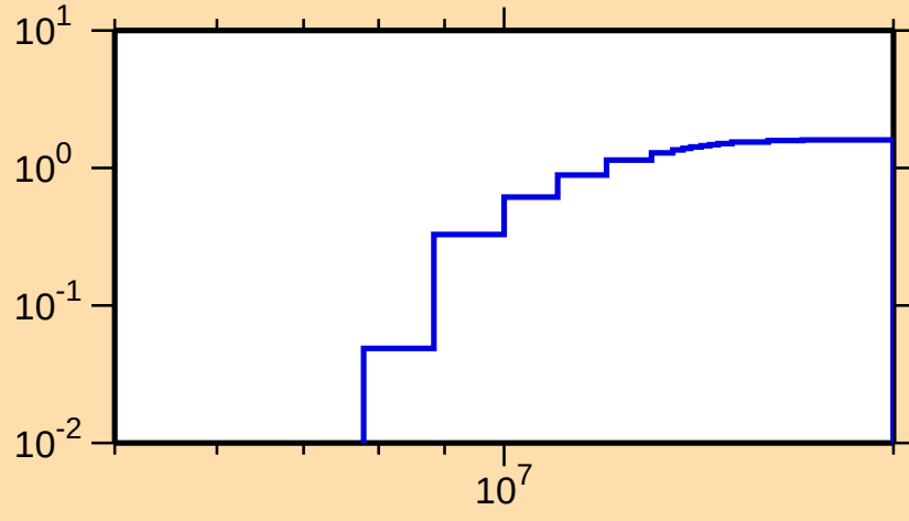
\sigma vs. E for ^{170}\text{Ta}(n,2n)
