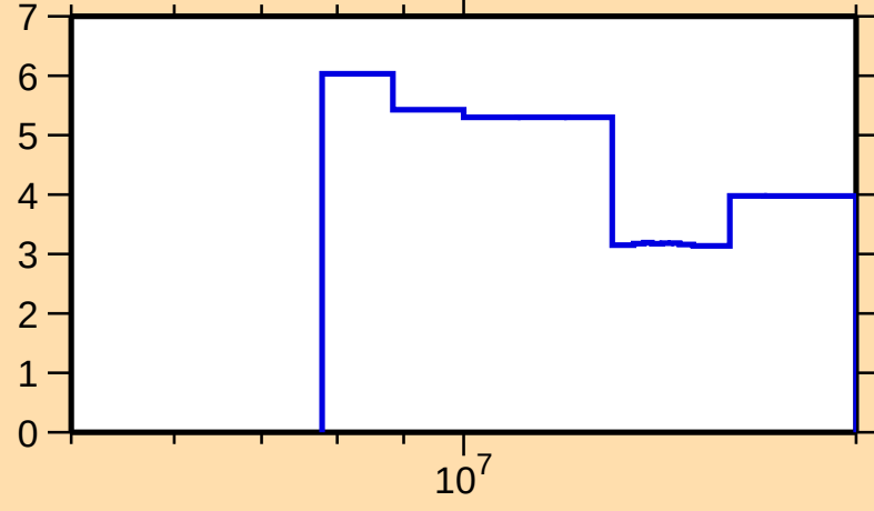
\Delta\sigma/\sigma vs. E for ^{170}\text{Ta}(n,\text{nonel.})
