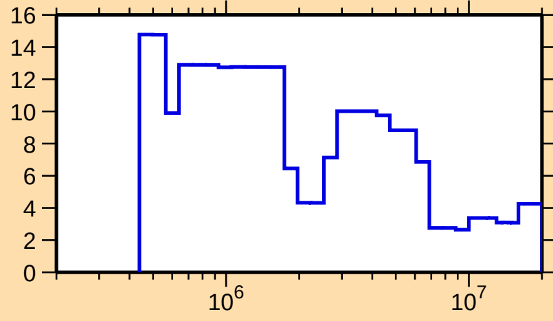
\Delta\sigma/\sigma vs. E for ^{170}\text{Ta}(n,\text{tot.})
