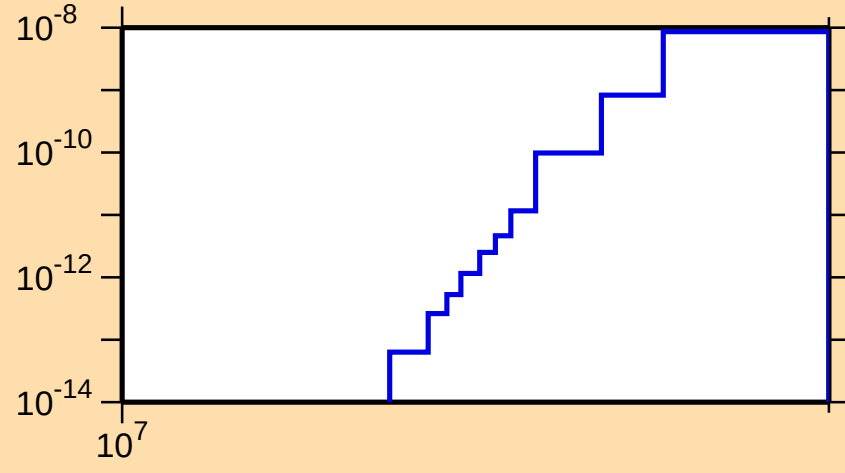
\sigma vs. E for ^{170}\text{Ta}(n,\text{pd})
