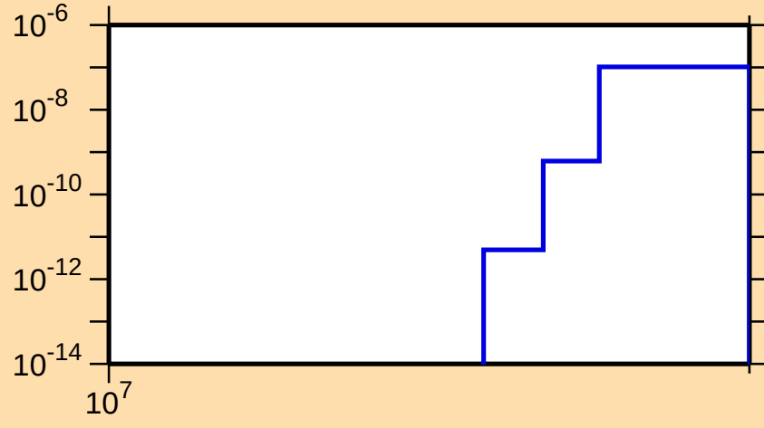
\sigma vs. E for ^{170}\text{Ta}(n,nt)
