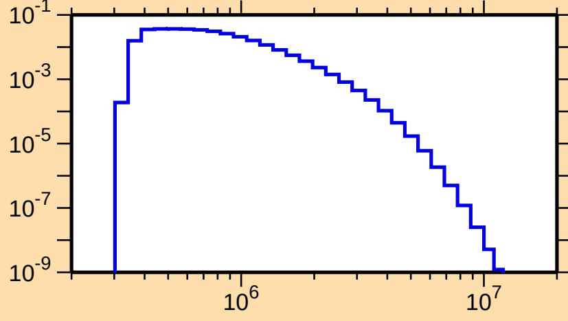
\sigma vs. E for ^{170}\text{Ta}(n,n_3)
