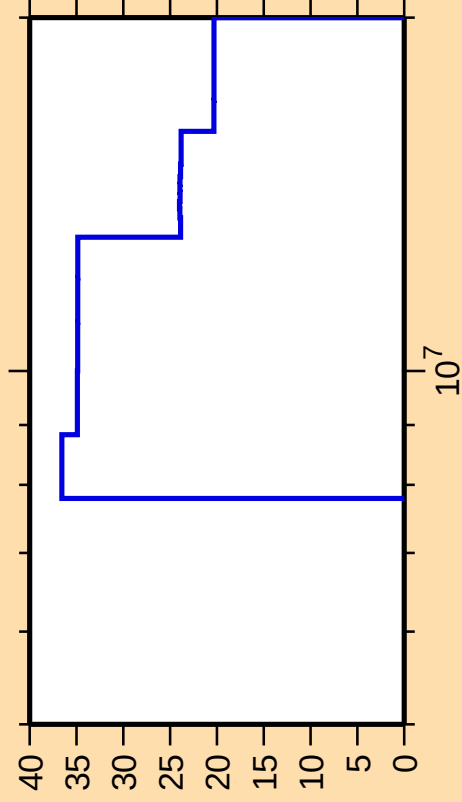
\Delta\sigma/\sigma vs. E for ^{170}\text{Ta}(n,2n)
