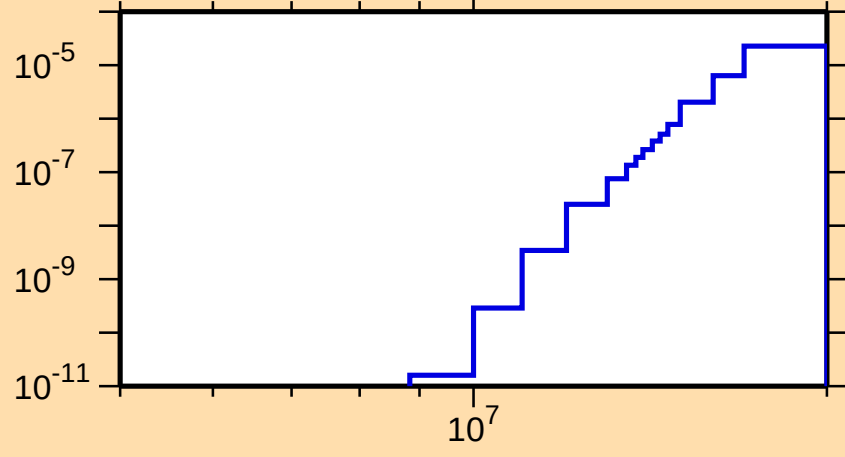
\sigma vs. E for ^{170}\text{Ta}(n,\text{He3})
