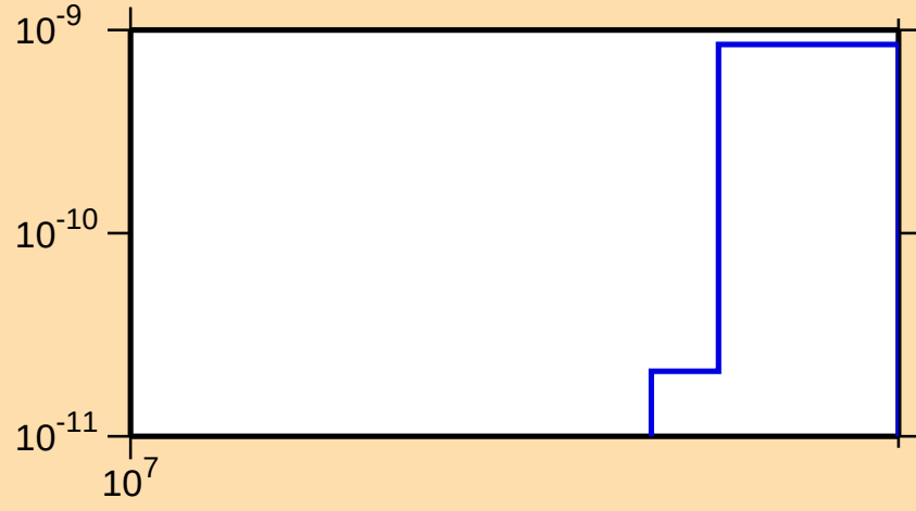
\sigma vs. E for ^{170}\text{Ta}(n,\text{pt})
