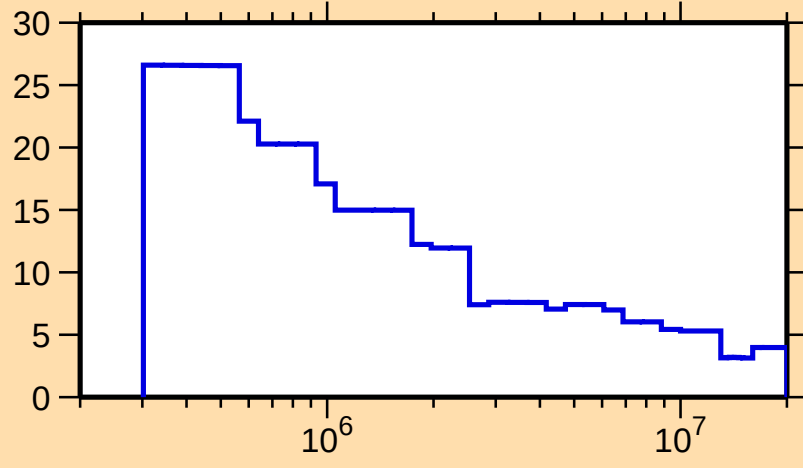
\Delta\sigma/\sigma vs. E for ^{170}\text{Ta}(n,\text{nonel.})
