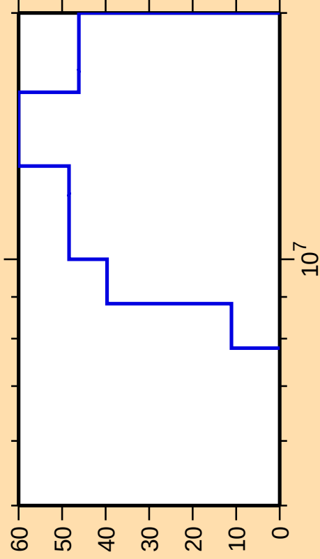
\Delta\sigma/\sigma vs. E for ^{170}\text{Ta}(n,n\text{cont.})
