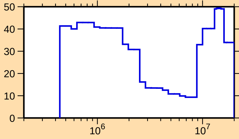
\Delta\sigma/\sigma vs. E for ^{170}\text{Ta}(n,\text{inel.})
