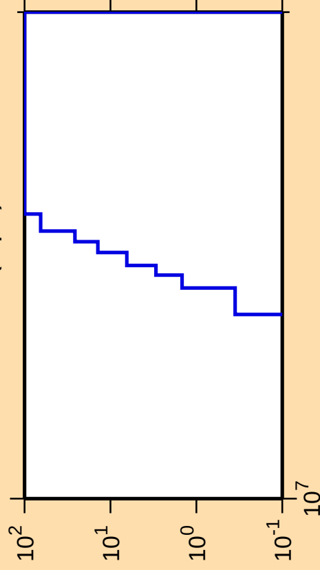
\Delta\sigma/\sigma vs. E for ^{170}\text{Ta}(n,\text{pd})
