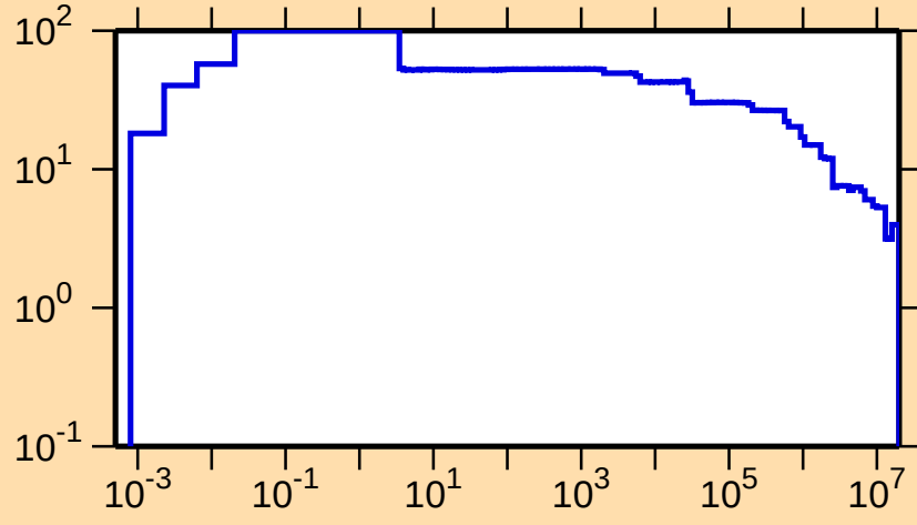
\Delta\sigma/\sigma vs. E for ^{170}\text{Ta}(n,\text{nonel.})
