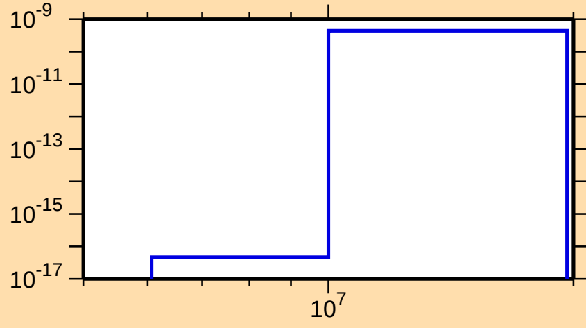
\sigma vs. E for ^{170}\text{Ta}(\text{mt117})
