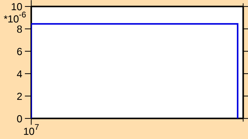
\sigma vs. E for ^{170}\text{Ta}(n,3n)
