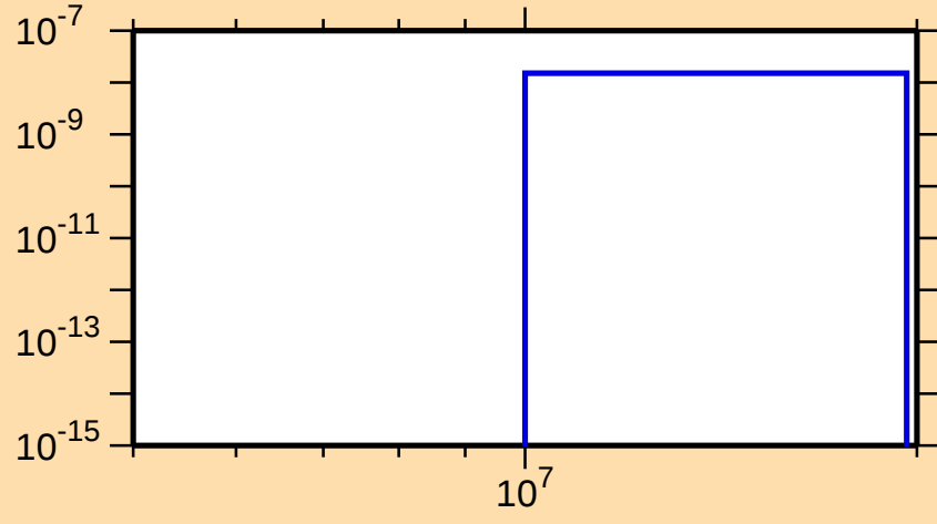
\sigma vs. E for ^{170}\text{Ta}(\text{mt } 45)
