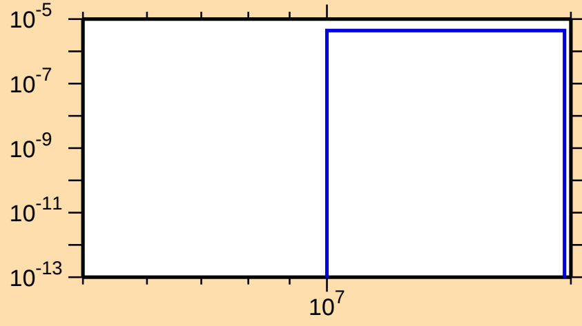
\sigma vs. E for ^{170}\text{Ta}(n,\text{nd})
