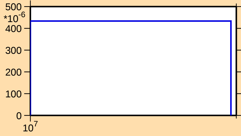
\sigma vs. E for ^{170}\text{Ta}(n,2np)
