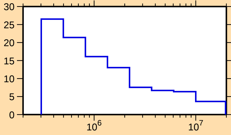
\Delta\sigma/\sigma vs. E for ^{170}\text{Ta}(n,n\text{onel.})
