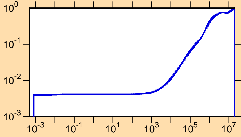
\mu vs. E for ^{171}\text{Ta}(\text{mt251})
