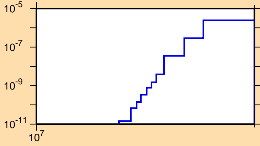
\sigma vs. E for ^{171}\text{Ta}(n,2n\alpha)
