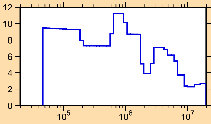
\Delta\sigma/\sigma vs. E for ^{171}\text{Ta}(n,\text{tot.})
