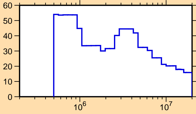
\Delta\sigma/\sigma vs. E for ^{171}\text{Ta}(n,n_1)
