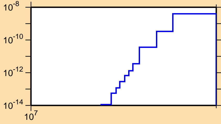
\sigma vs. E for ^{171}\text{Ta}(n,pd)
