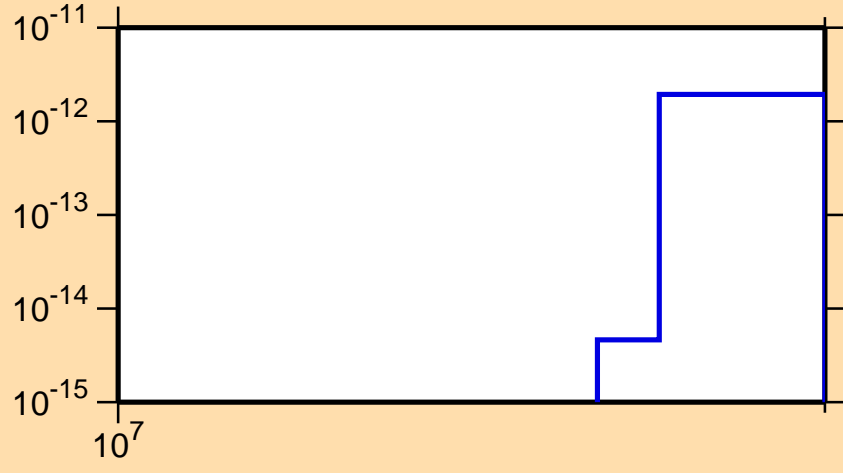
\sigma vs. E for ^{171}\text{Ta} (mt 34)
