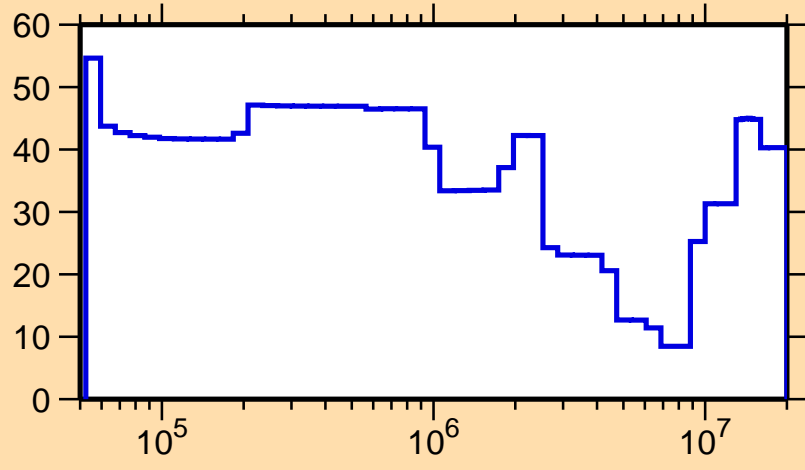
\Delta\sigma/\sigma vs. E for ^{171}\text{Ta}(n,\text{inel.})
