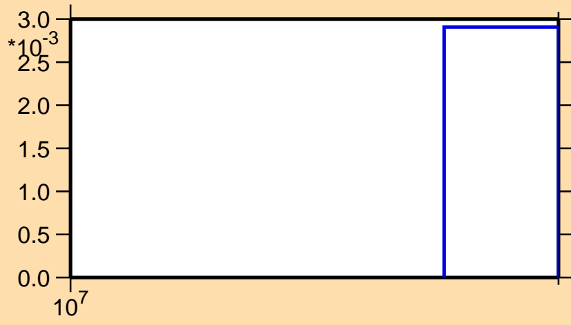
\sigma vs. E for ^{171}\text{Ta}(n,3n)
