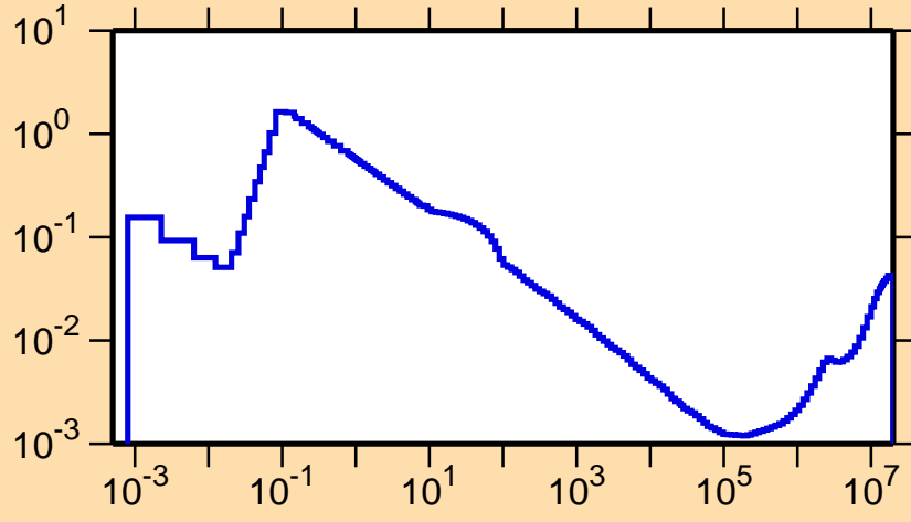
\sigma vs. E for ^{171}\text{Ta}(n,p)
