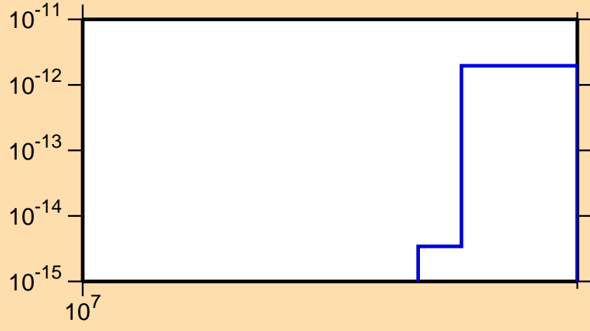
\sigma vs. E for ^{171}\text{Ta}(n,\text{pt})
