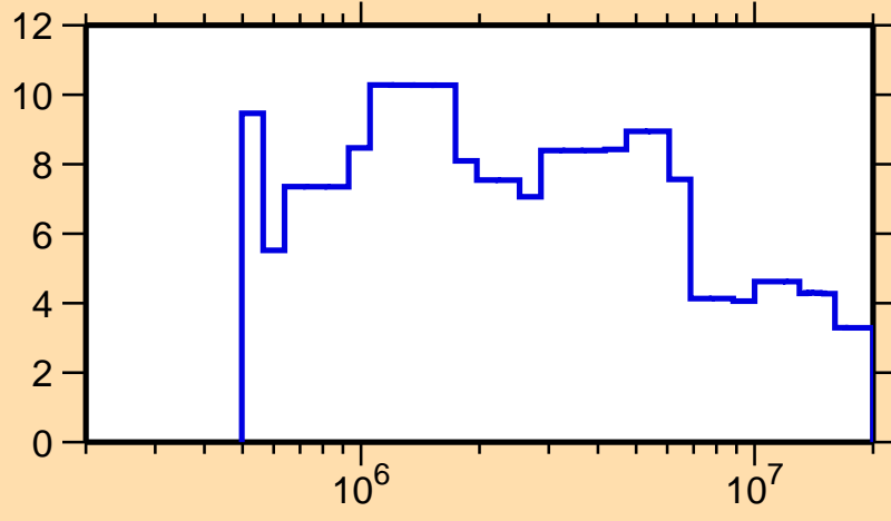
\Delta\sigma/\sigma vs. E for ^{171}\text{Ta}(n,\text{el.})
