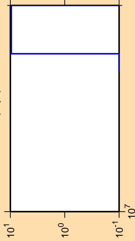
\Delta\sigma/\sigma vs. E for ^{171}\text{Ta}(n,\text{pt})
