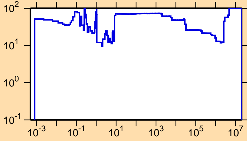
\Delta\sigma/\sigma vs. E for ^{171}\text{Ta}(n,\gamma)
