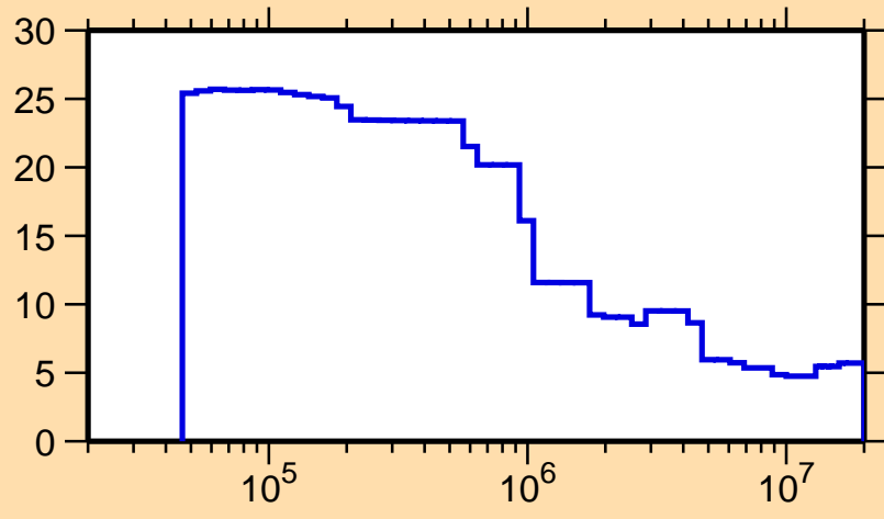
\Delta\sigma/\sigma vs. E for ^{171}\text{Ta}(n,\text{nonel.})
