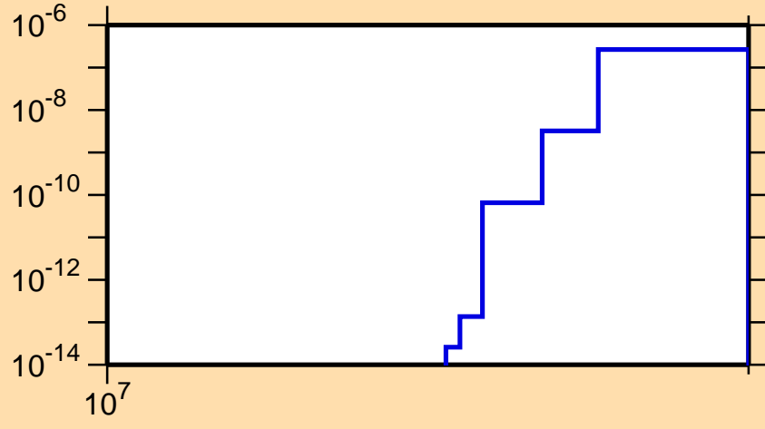
\sigma vs. E for ^{171}\text{Ta}(n,nt)
