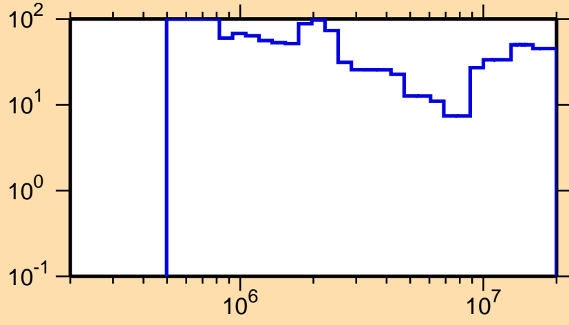
\Delta\sigma/\sigma vs. E for ^{171}\text{Ta}(n,n\text{cont.})
