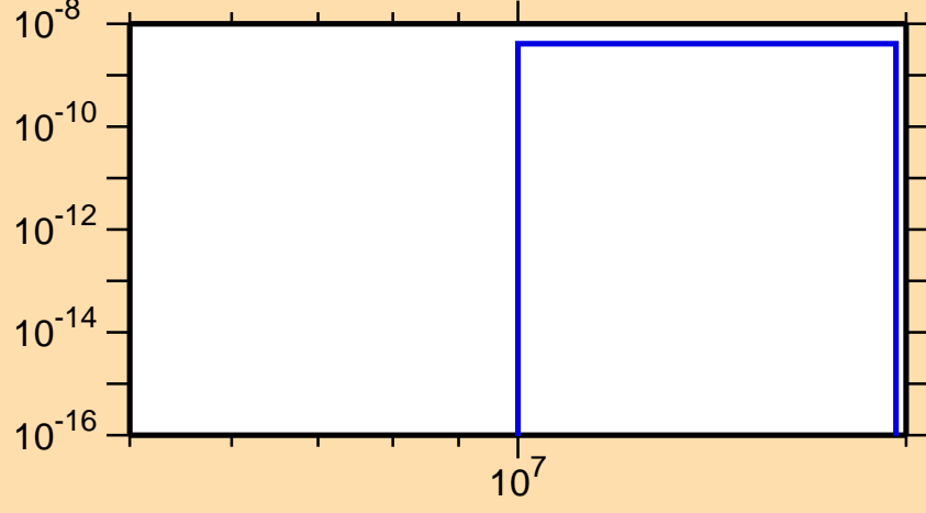
\sigma vs. E for ^{171}\text{Ta}(\text{mt } 45)
