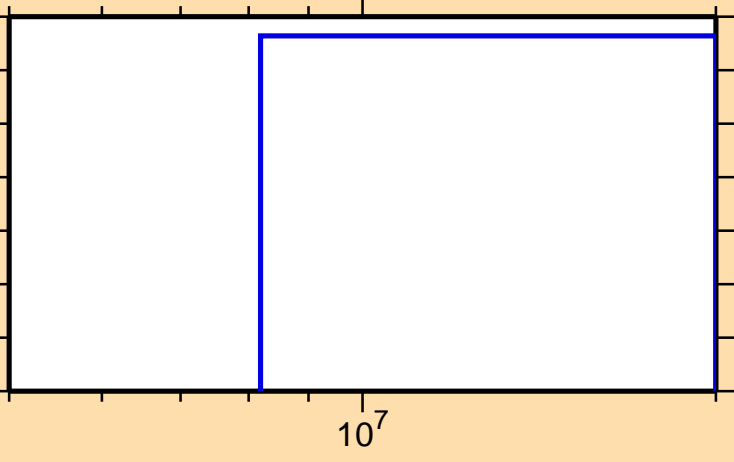
\sigma vs. E for ^{171}\text{Ta} (mt 45)
