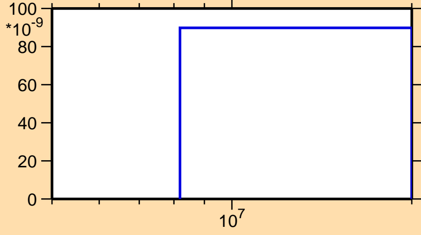
\sigma vs. E for ^{171}\text{Ta}(n,\text{nd})
