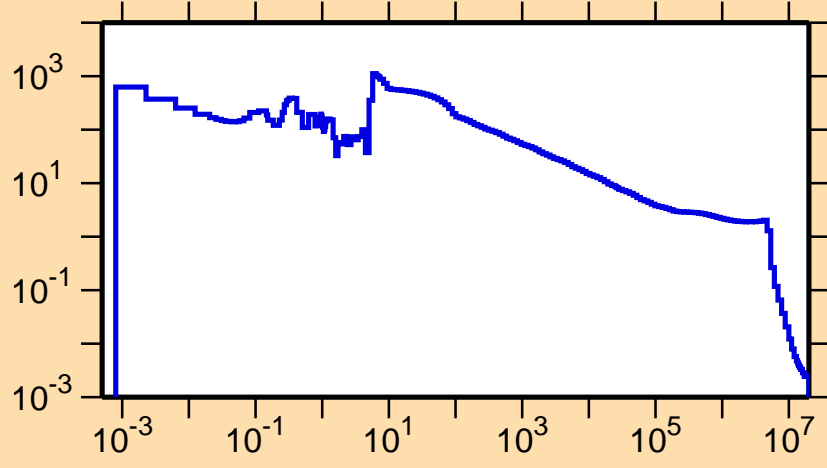
\sigma vs. E for ^{172}\text{Ta}(n,\gamma)
