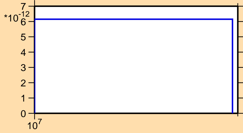
\sigma vs. E for ^{172}\text{Ta}(n,pd)
