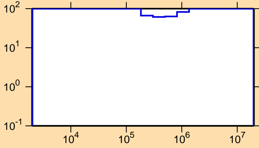
\Delta\sigma/\sigma vs. E for ^{172}\text{Ta}(n,n_1)
