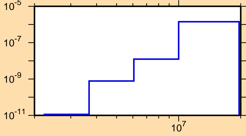
\sigma vs. E for ^{172}\text{Ta}(n,p\alpha)
