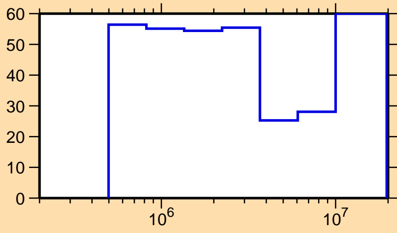
\Delta\sigma/\sigma vs. E for ^{172}\text{Ta}(n,n\text{cont.})
