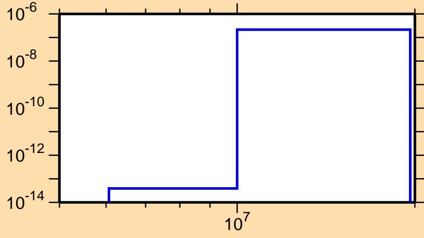
\sigma vs. E for ^{172}\text{Ta}(n,\text{He3})
