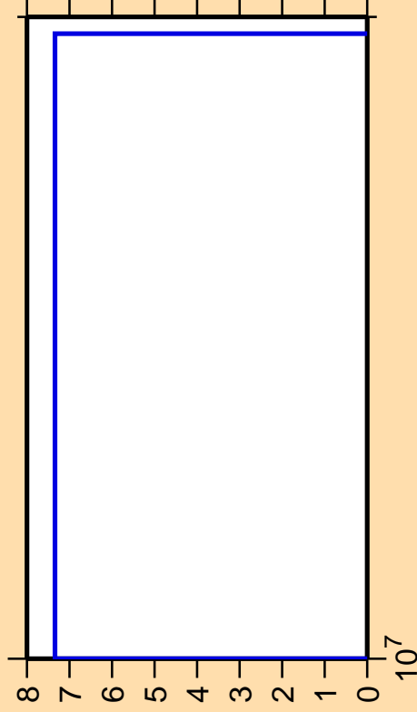
\Delta\sigma/\sigma vs. E for ^{172}\text{Ta} (mt 34)
