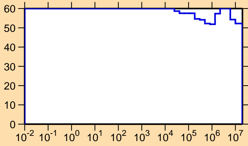
\Delta\sigma/\sigma vs. E for ^{172}\text{Ta}(n,p)
