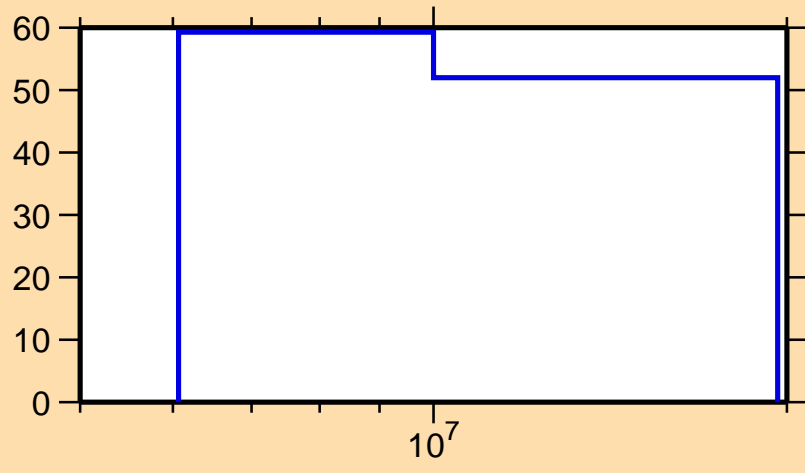
\Delta\sigma/\sigma vs. E for ^{172}\text{Ta}(n,2n)
