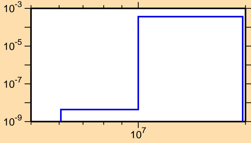
\sigma vs. E for ^{172}\text{Ta}(n,t)
