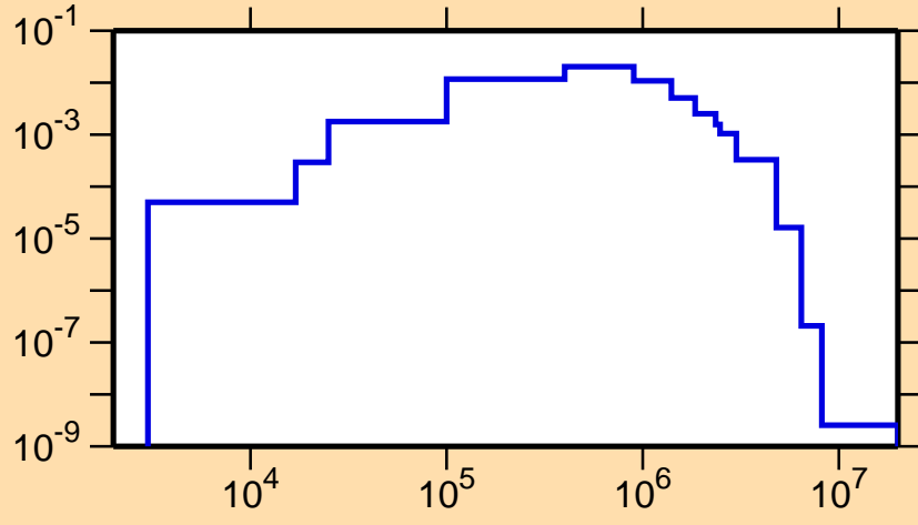
\sigma vs. E for ^{172}\text{Ta}(n,n_1)
