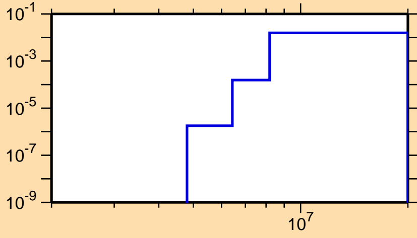
\sigma vs. E for ^{172}\text{Ta}(n,np)
