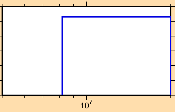
\sigma vs. E for ^{172}\text{Ta}(n,pd)
