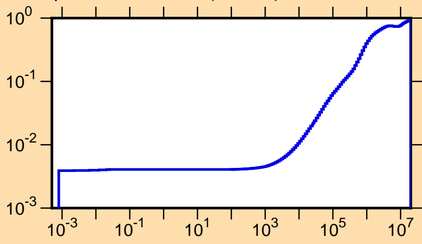
\mu vs. E for ^{173}\text{Ta}(\text{mt251})
