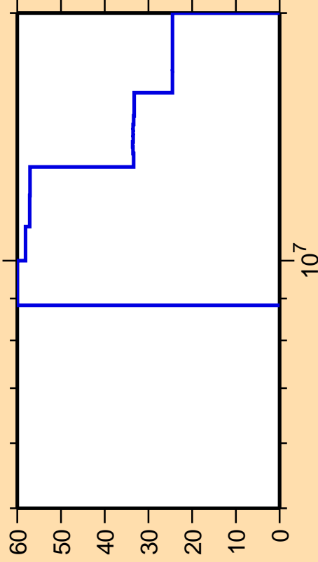
\Delta\sigma/\sigma vs. E for ^{173}\text{Ta}(n,2n)
