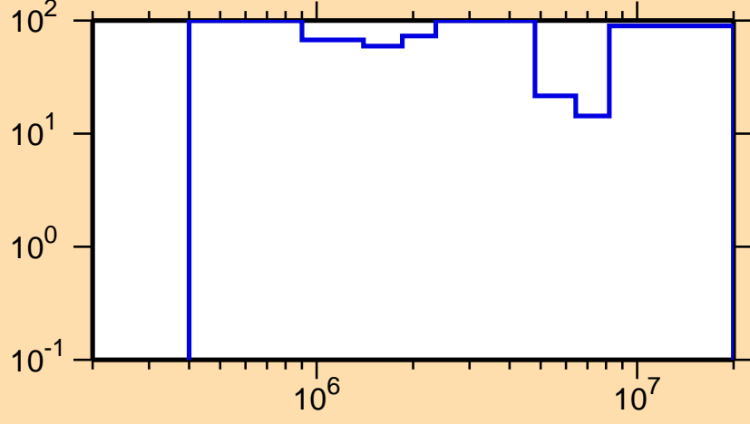
\Delta\sigma/\sigma vs. E for ^{173}\text{Ta}(n,n\text{cont.})
