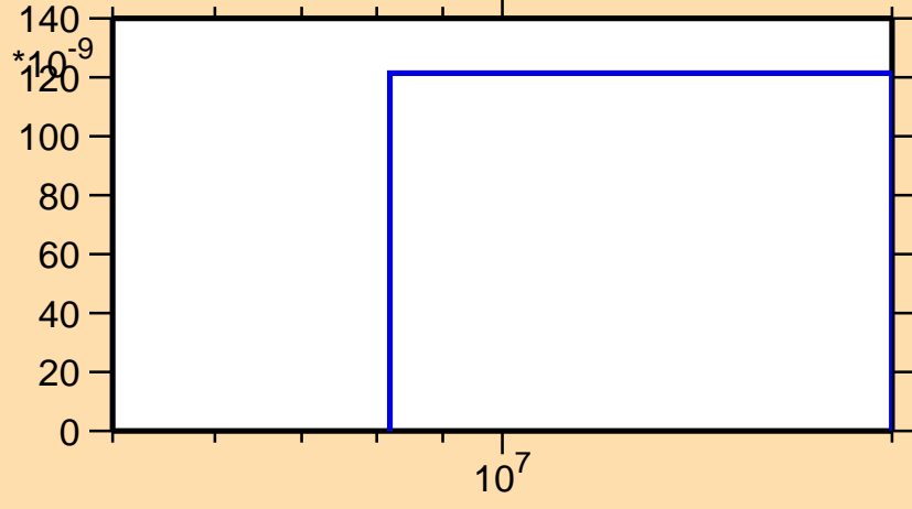
\sigma vs. E for ^{173}\text{Ta}(n,\text{nd})
