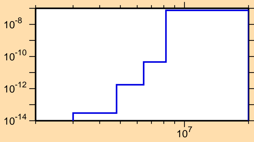
\sigma vs. E for ^{173}\text{Ta}(n,p\alpha)
