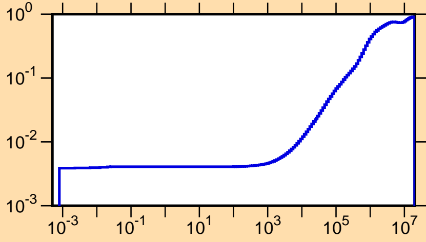
\mu vs. E for ^{174}\text{Ta}(\text{mt251})
