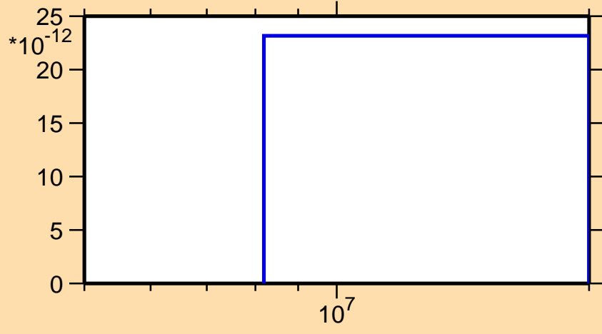
\sigma vs. E for ^{174}\text{Ta} (mt 45)
