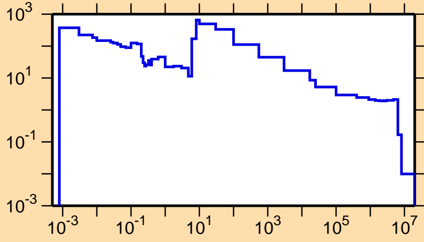
\sigma vs. E for ^{174}\text{Ta}(n,\gamma)
