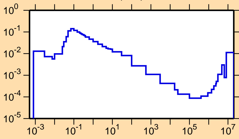
\sigma vs. E for ^{174}\text{Ta}(n,\alpha)
