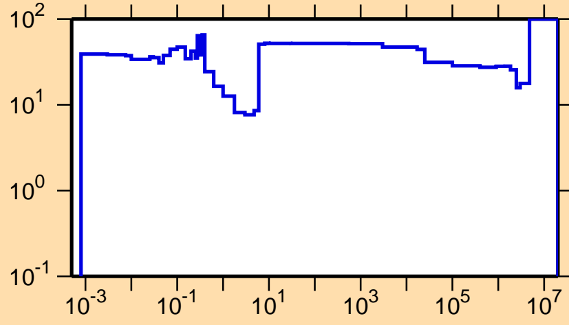
\Delta\sigma/\sigma vs. E for ^{174}\text{Ta}(n,\gamma)
