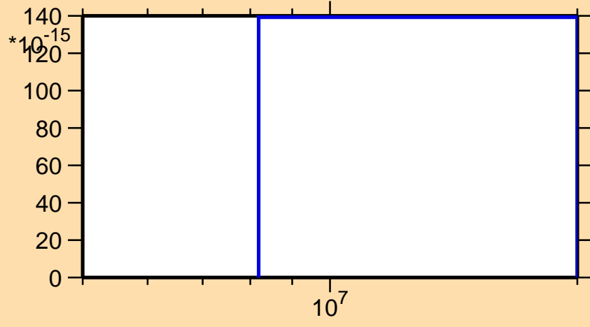
\sigma vs. E for ^{174}\text{Ta}(n,pd)
