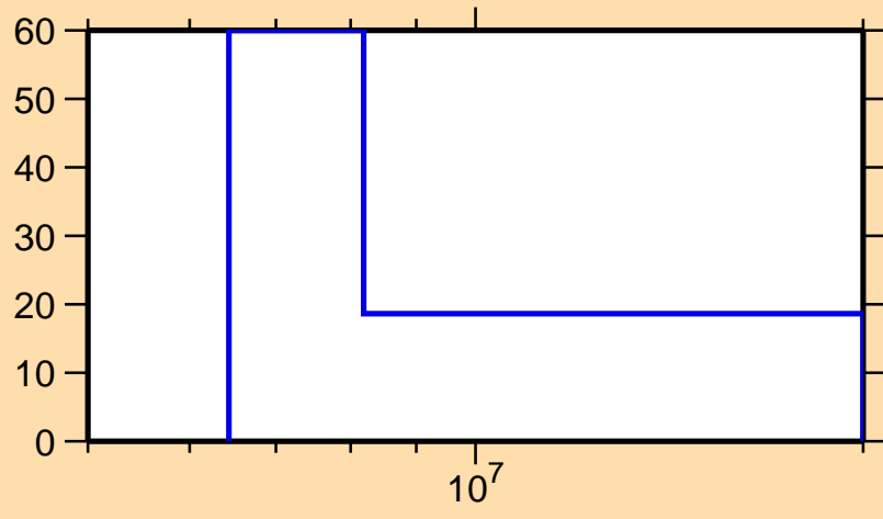
\Delta\sigma/\sigma vs. E for ^{174}\text{Ta}(n,2n)
