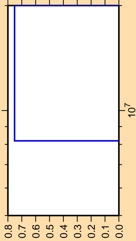
\Delta\sigma/\sigma vs. E for ^{174}\text{Ta}(n,pd)
