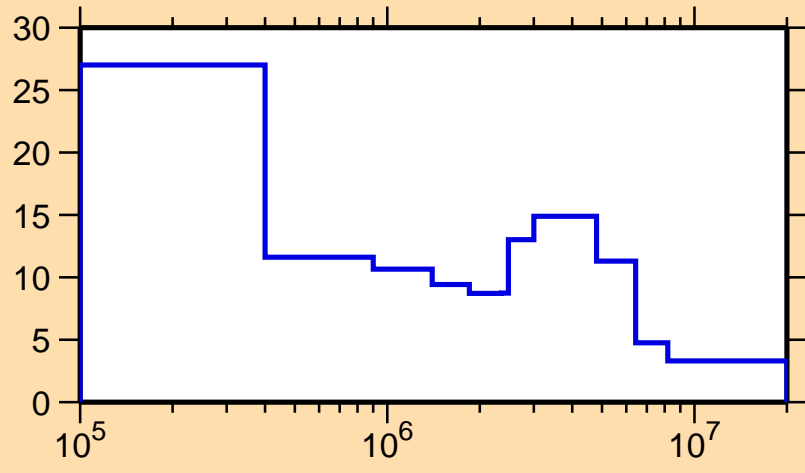
\Delta\sigma/\sigma vs. E for ^{174}\text{Ta}(n,tot.)
