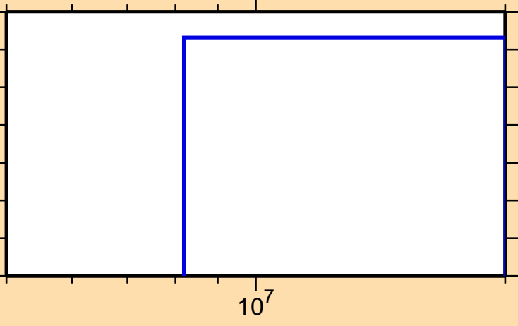
\sigma vs. E for ^{174}\text{Ta} (mt 42)
