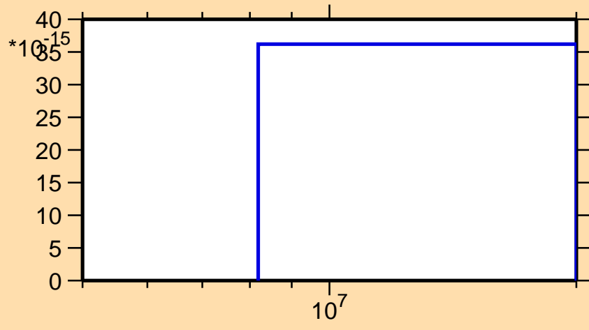
\sigma vs. E for ^{174}\text{Ta}(n,\text{pt})
