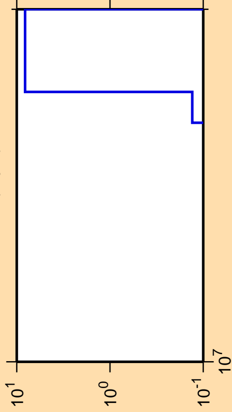
\Delta\sigma/\sigma vs. E for ^{175}\text{Ta}(n,pd)
