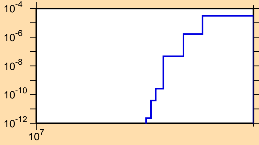
\sigma vs. E for ^{175}\text{Ta}(n,2np)
