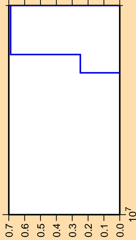
\Delta\sigma/\sigma vs. E for ^{175}\text{Ta}(n,3n\alpha)
