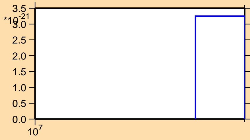
\sigma vs. E for ^{175}\text{Ta} (mt 42)
