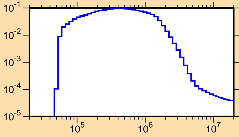
\sigma vs. E for ^{175}\text{Ta}(n,n_2)
