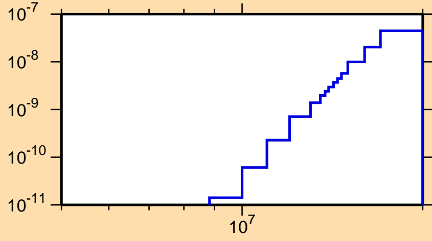
\sigma vs. E for ^{175}\text{Ta}(n,p\alpha)
