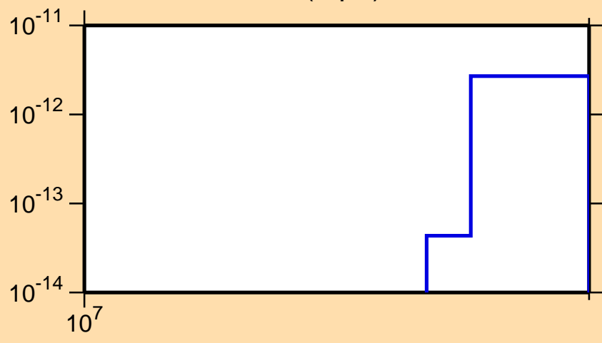
\sigma vs. E for ^{175}\text{Ta}(n,pd)
