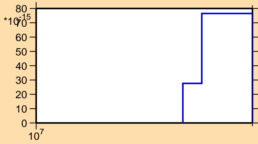
\sigma vs. E for ^{175}\text{Ta}(n,3n\alpha)
