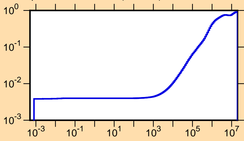
\mu vs. E for ^{176}\text{Ta}(\text{mt251})
