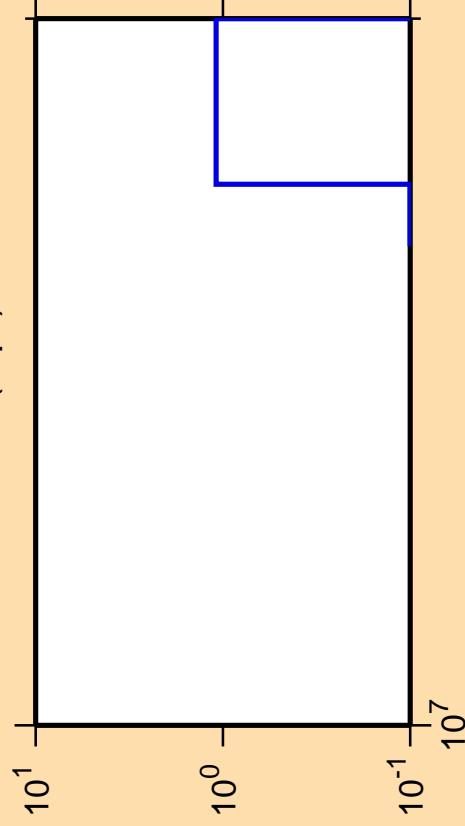
\Delta\sigma/\sigma vs. E for ^{176}\text{Ta}(n,\text{pt})
