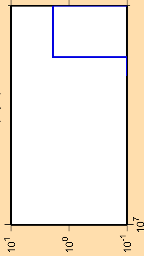
\Delta\sigma/\sigma vs. E for ^{176}\text{Ta}(n,pd)
