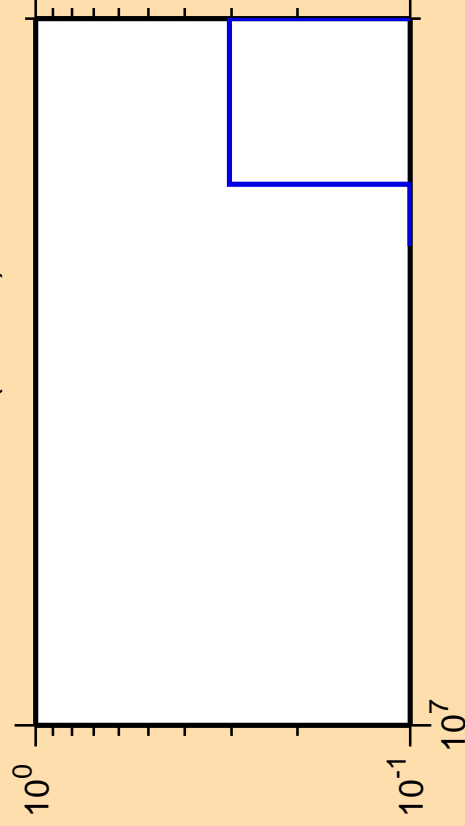
\Delta\sigma/\sigma vs. E for ^{176}\text{Ta}(n,3n\alpha)
