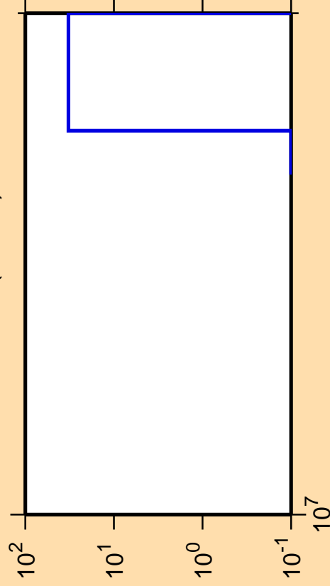
\Delta\sigma/\sigma vs. E for ^{176}\text{Ta} (mt 34)
