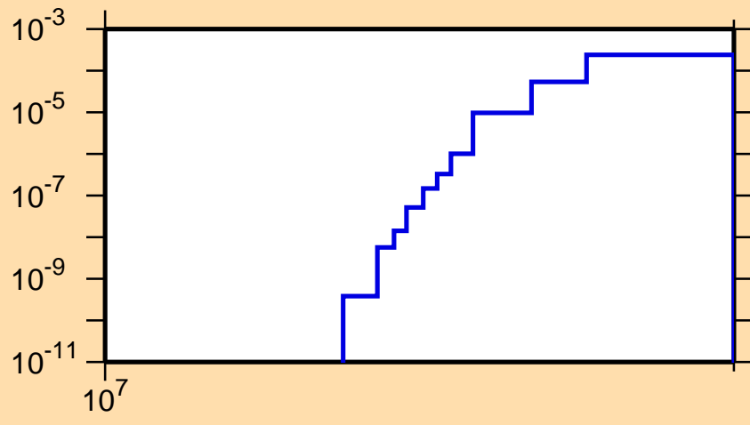
\sigma vs. E for ^{176}\text{Ta}(n,2np)
