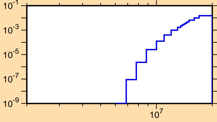
\sigma vs. E for ^{176}\text{Ta}(n,np)
