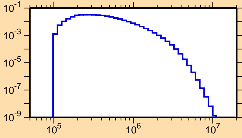
\sigma vs. E for ^{176}\text{Ta}(n,n_3)
