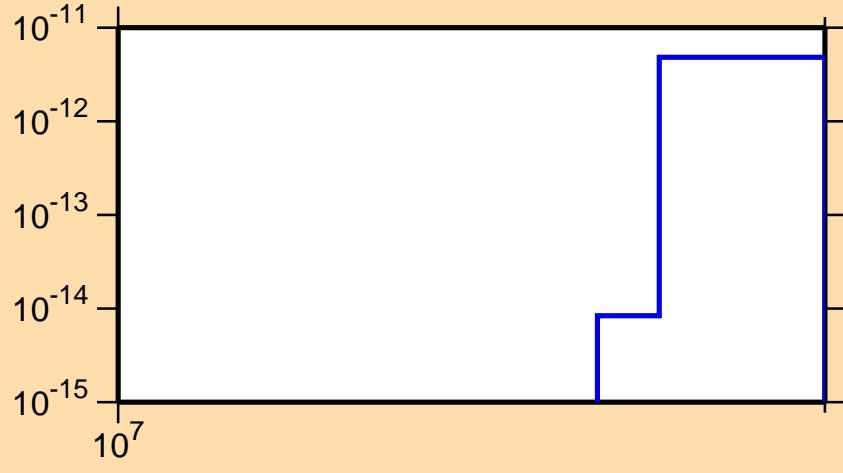
\sigma vs. E for ^{176}\text{Ta} (mt 34)
