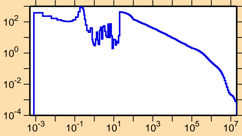
\sigma vs. E for ^{176}\text{Ta}(n,\gamma)
