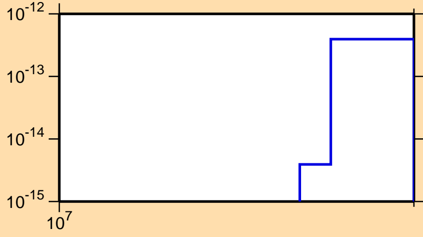
\sigma vs. E for ^{176}\text{Ta}(n,pd)
