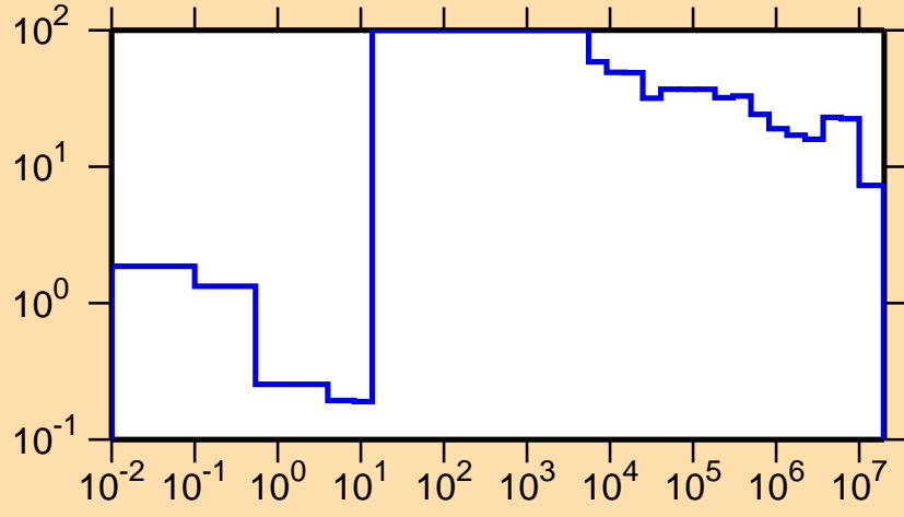
\Delta\sigma/\sigma vs. E for ^{176}\text{Ta}(n,el.)
