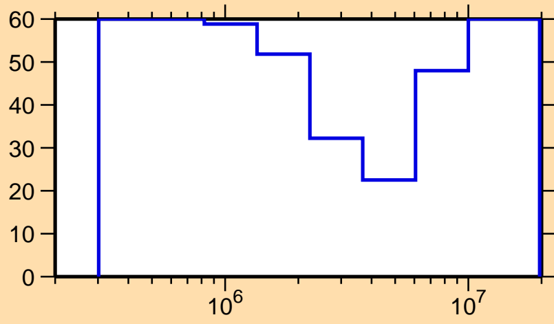
\Delta\sigma/\sigma vs. E for ^{176}\text{Ta}(n,n\text{cont.})
